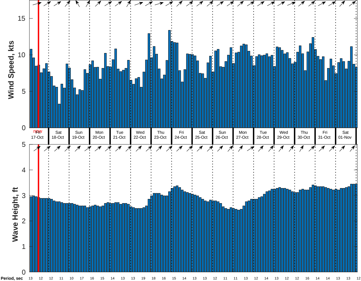
Wind & Wave Forecast for CSA (ONHYM) PPL EBS - Nigeria from 16-Oct-2025 02:00:00 to 01-Nov-2025 02:00:00
