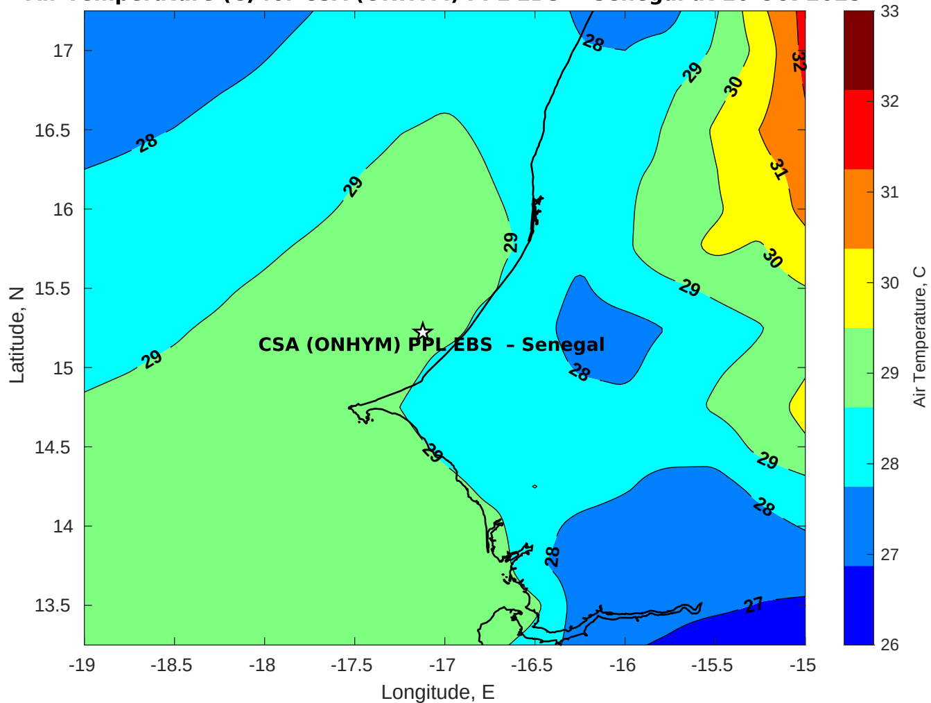
Air Temperature (C) for CSA (ONHYM) PPL EBS - Senegal at 16-Oct-2025
