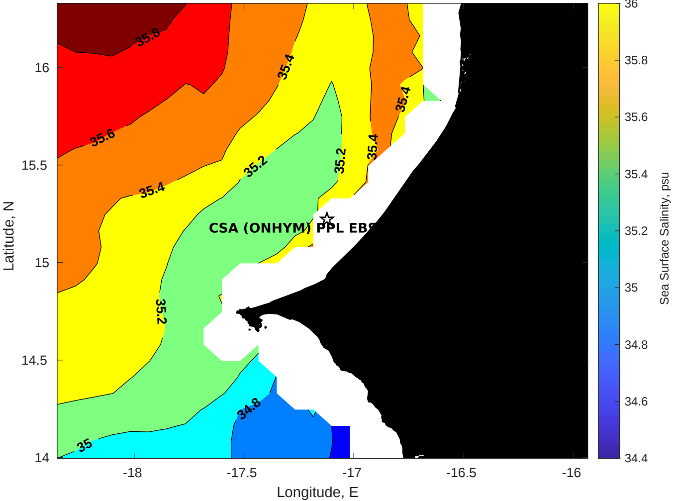
Surface Salinity for CSA (ONHYM) PPL EBS - Senegal at 13-Oct-2025 00:00:00
