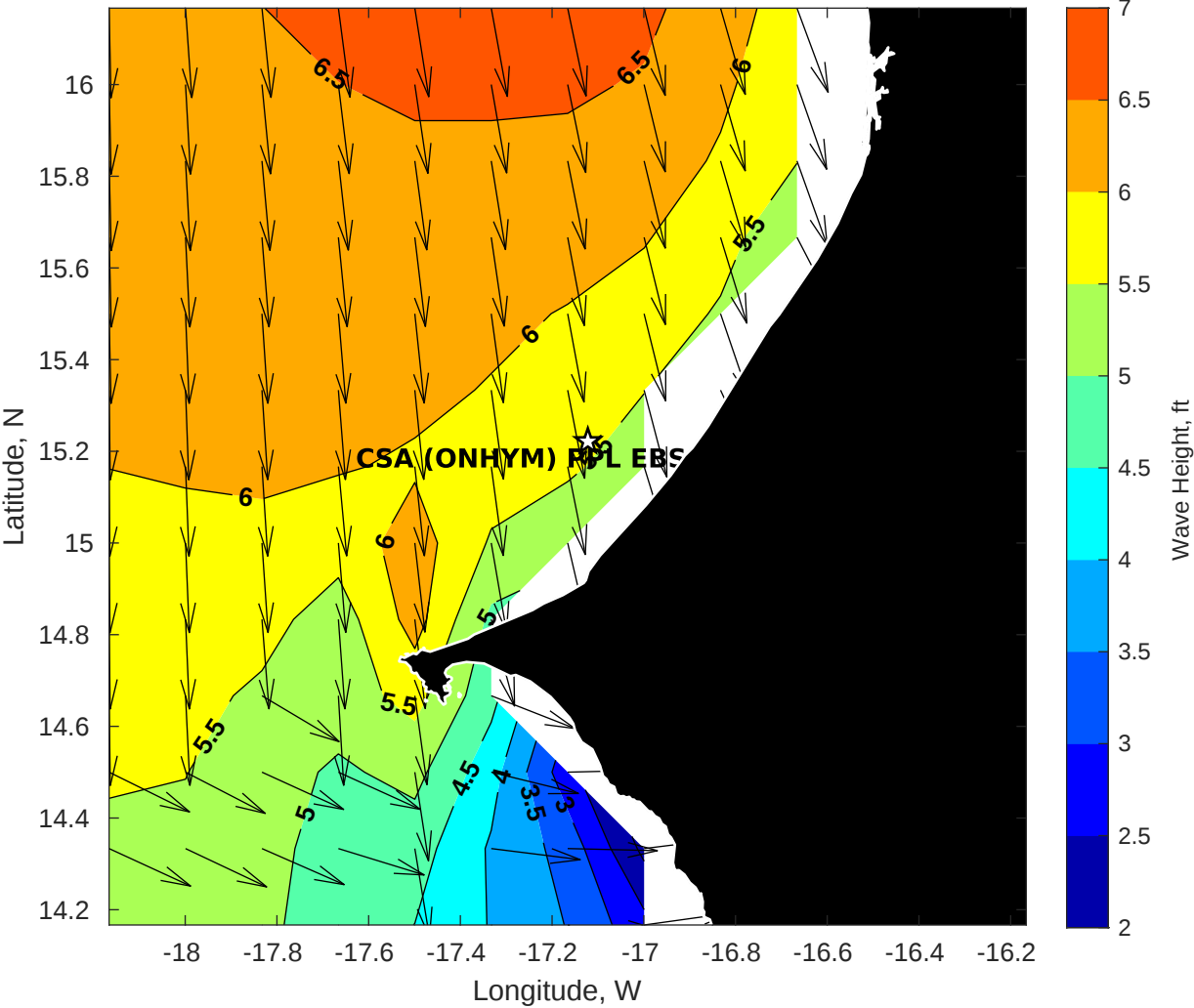
Wave Height (ft) for CSA (ONHYM) PPL EBS - Senegal at 16-Oct-2025 09:00:00
