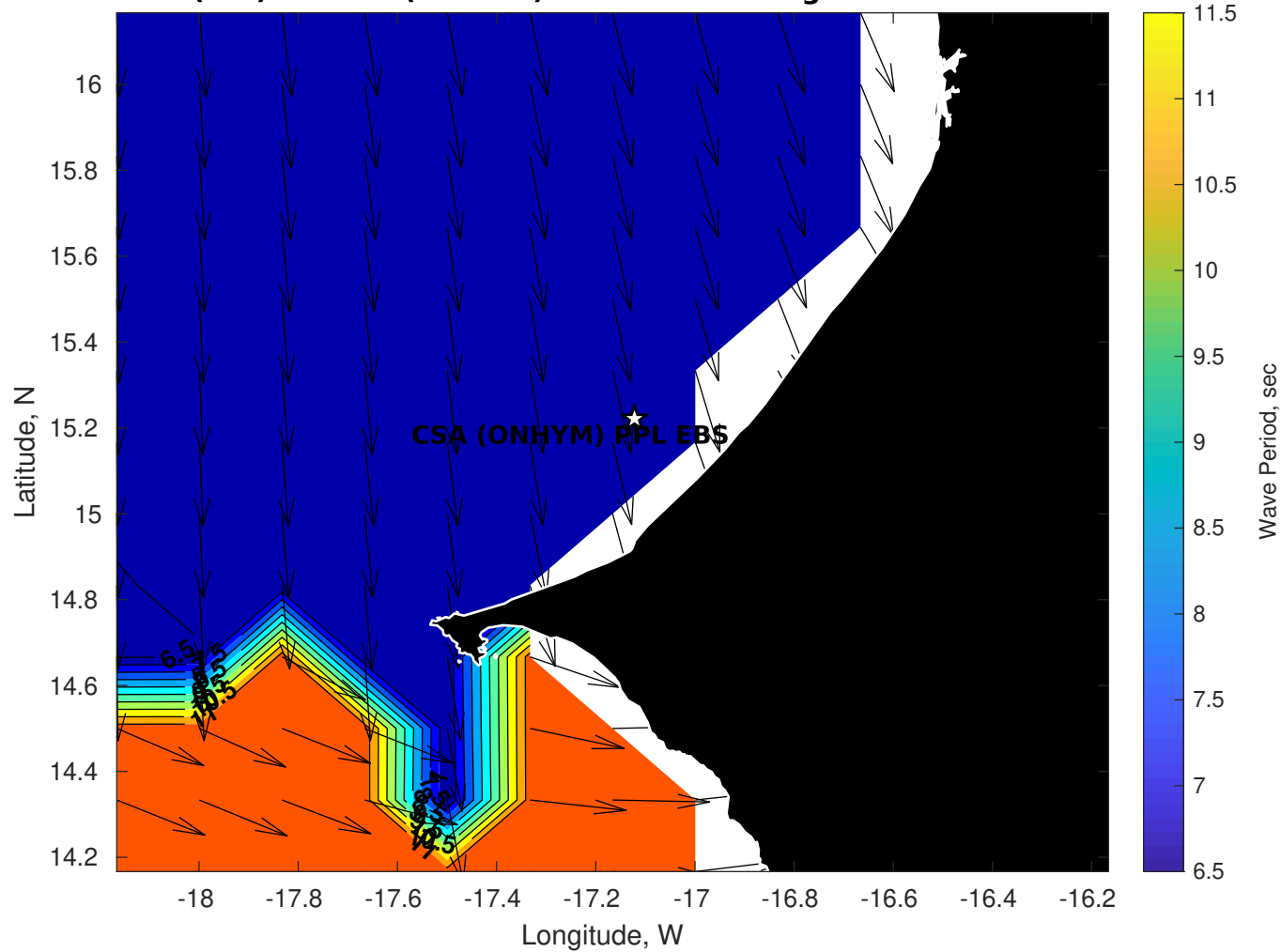
Wave Period (sec) for CSA (ONHYM) PPL EBS - Senegal at 16-Oct-2025 09:00:00
