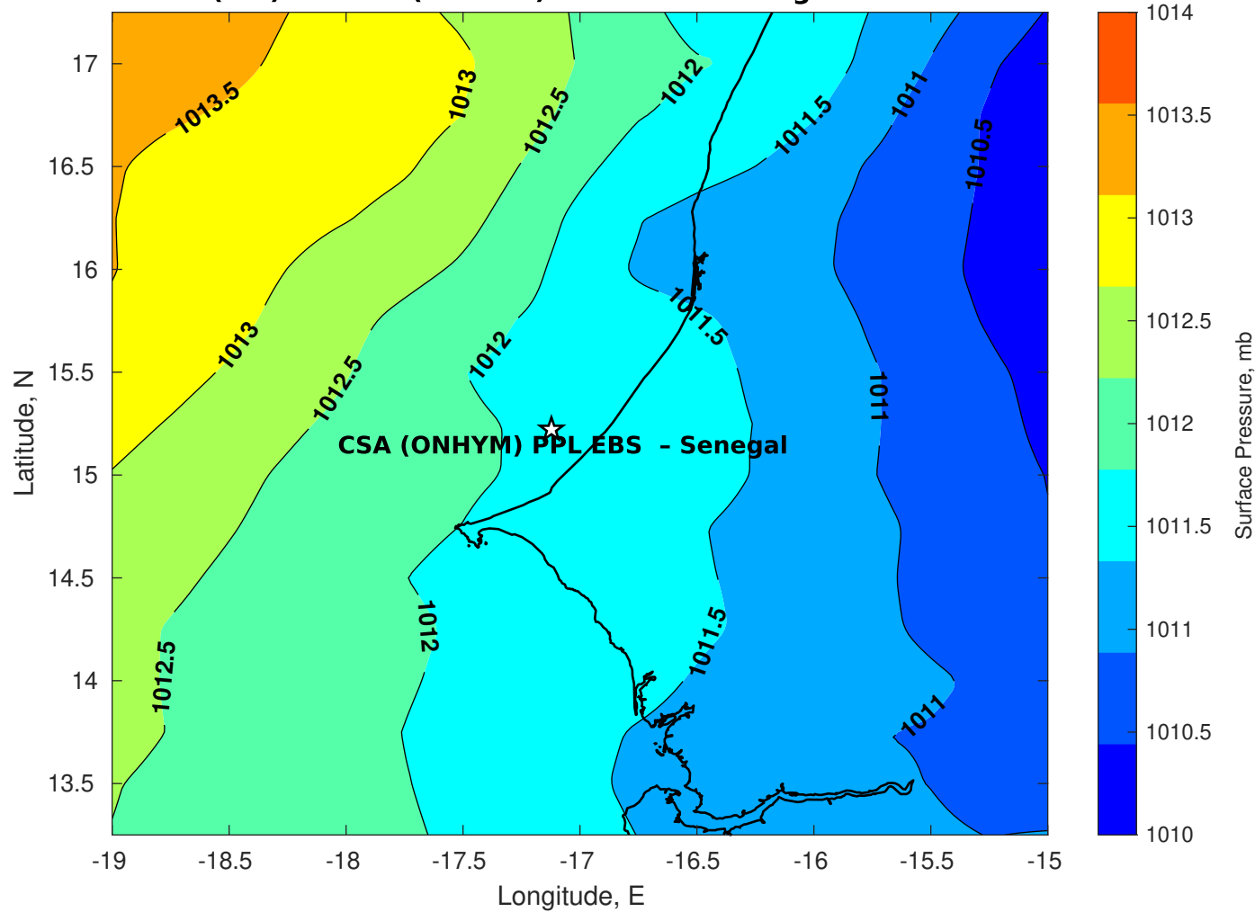
Surface Pressure (mb) for CSA (ONHYM) PPL EBS - Senegal at 16-Oct-2025 00:00:00
