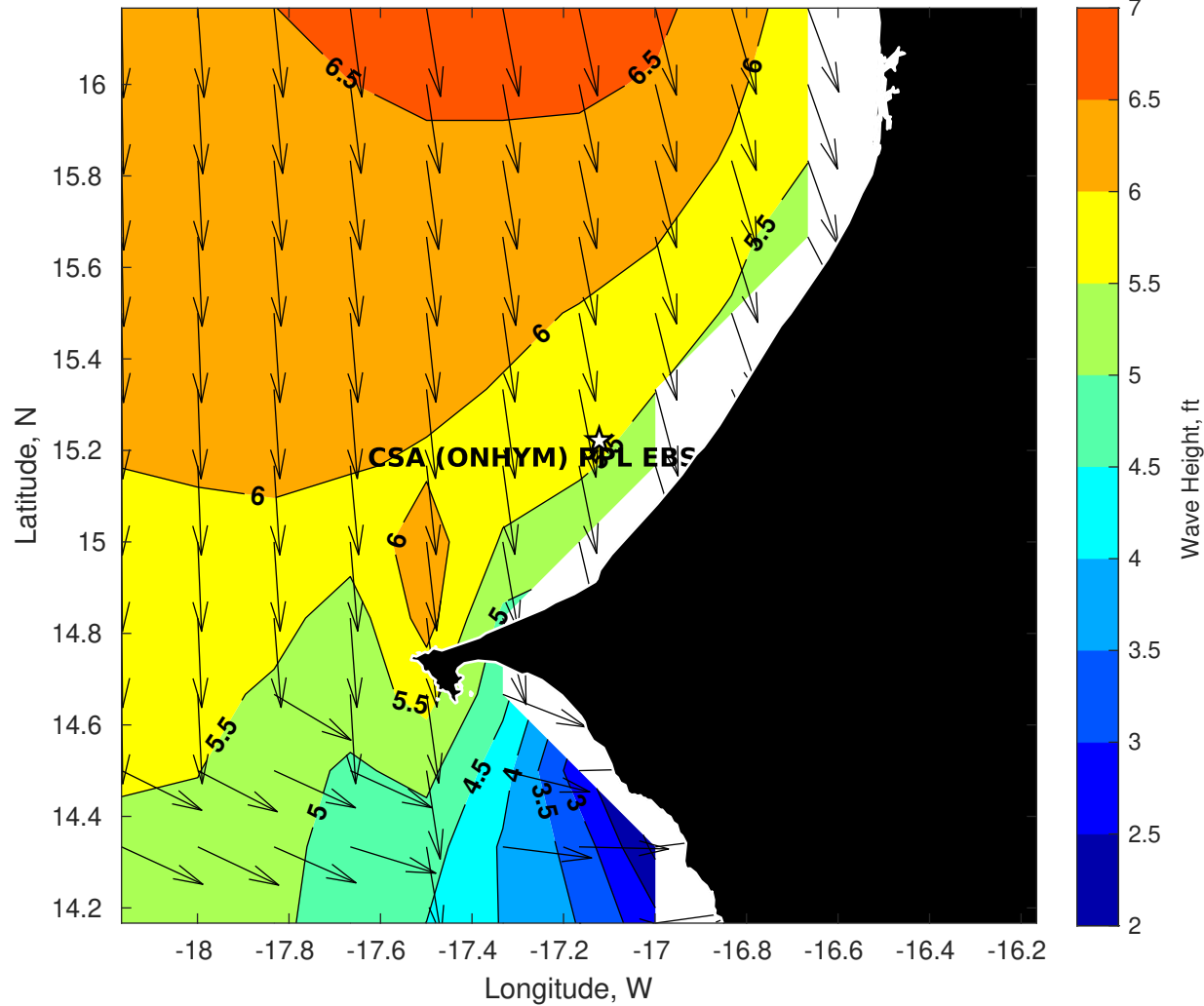
Wave Height (ft) for CSA (ONHYM) PPL EBS - Senegal at 16-Oct-2025 09:00:00
