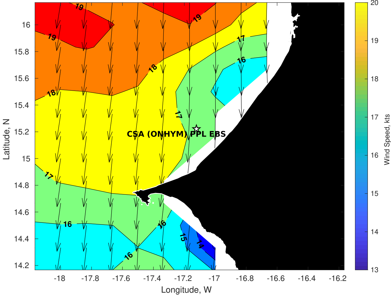
Winds (kts) for CSA (ONHYM) PPL EBS - Senegal at 16-Oct-2025 09:00:00
