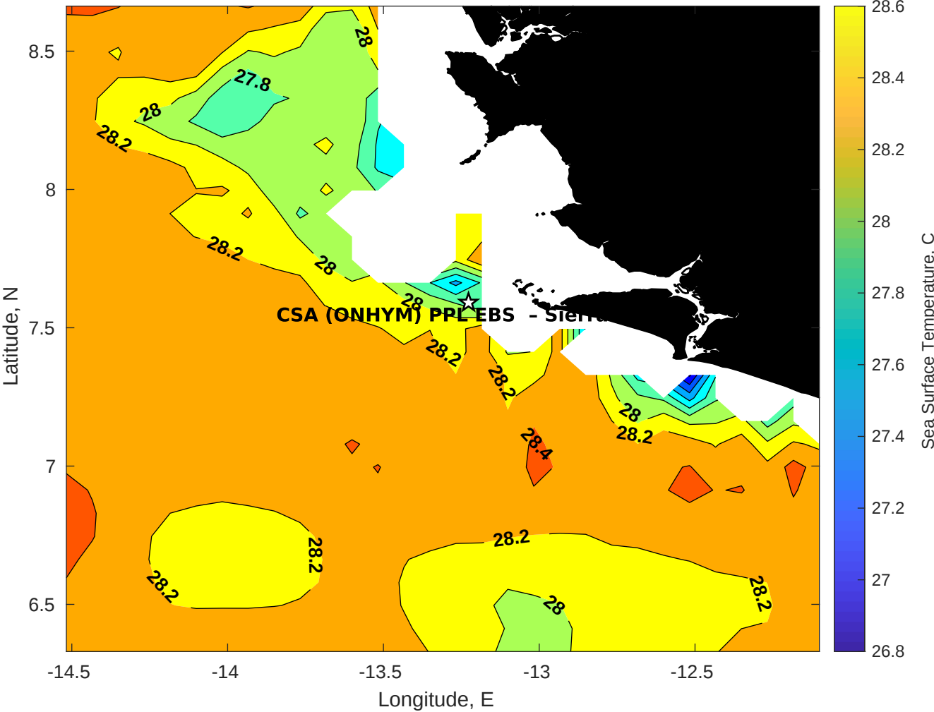
SST for CSA (ONHYM) PPL EBS - Sierra Leone at 15-Oct-2025 00:00:00
