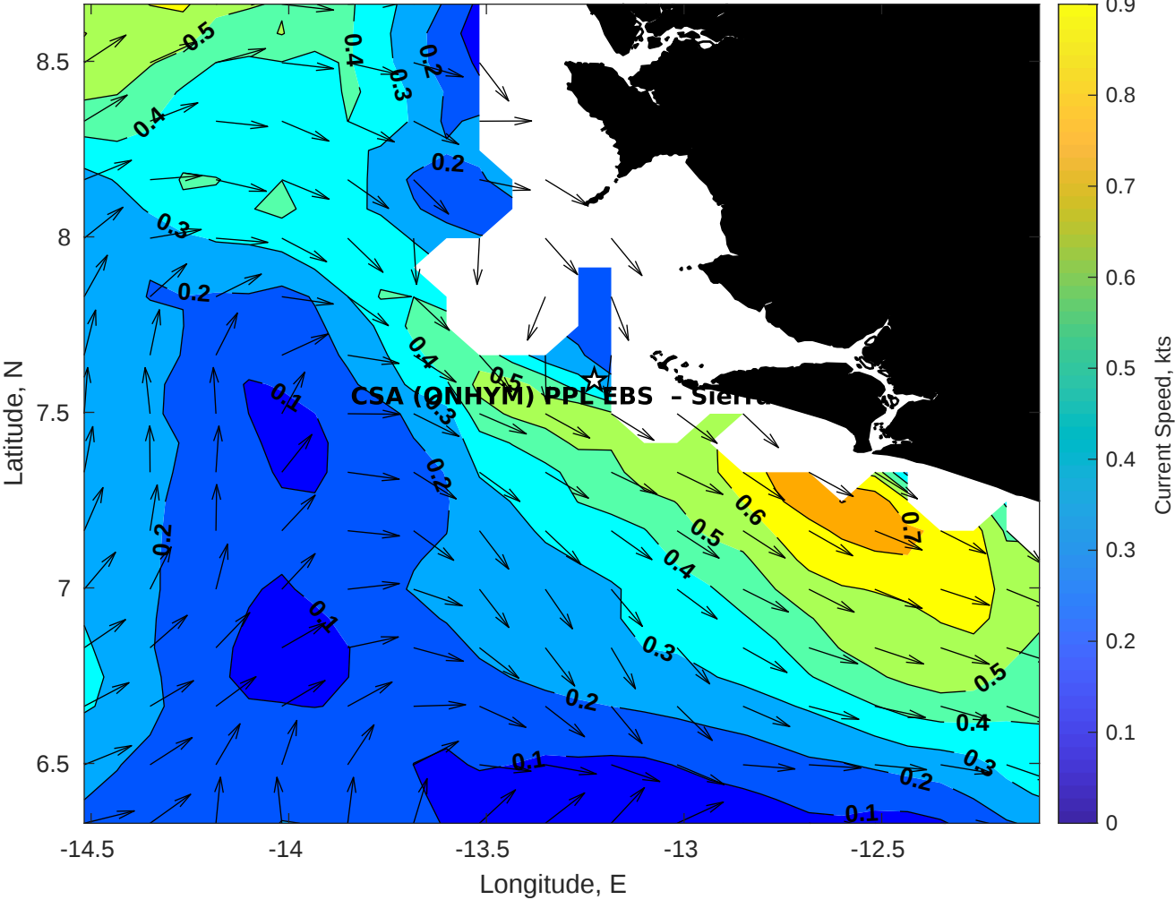
Surface Currents for CSA (ONHYM) PPL EBS - Sierra Leone at 15-Oct-2025 00:00:00
