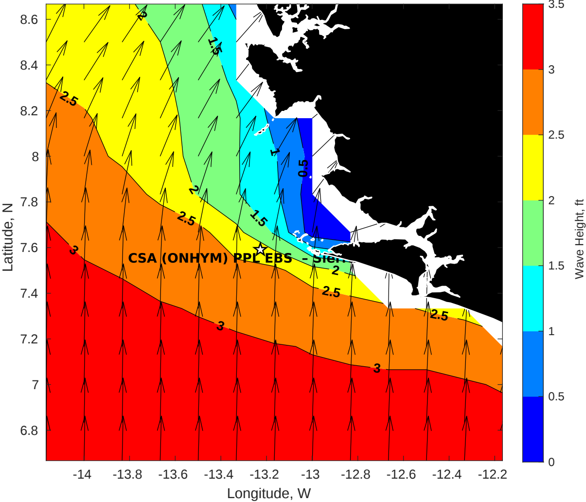
Wave Height (ft) for CSA (ONHYM) PPL EBS - Sierra Leone at 16-Oct-2025 09:00:00
