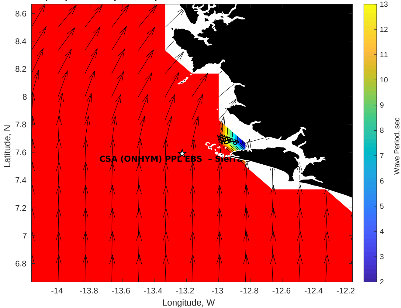
Wave Period (sec) for CSA (ONHYM) PPL EBS - Sierra Leone at 16-Oct-2025 09:00:00
