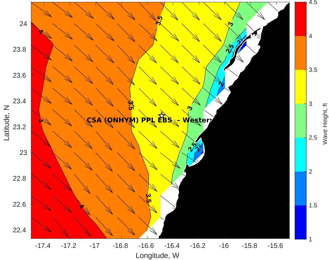
Wave Height (ft) for CSA (ONHYM) PPL EBS - Western Sahara at 16-Oct-2025 09:00:00
