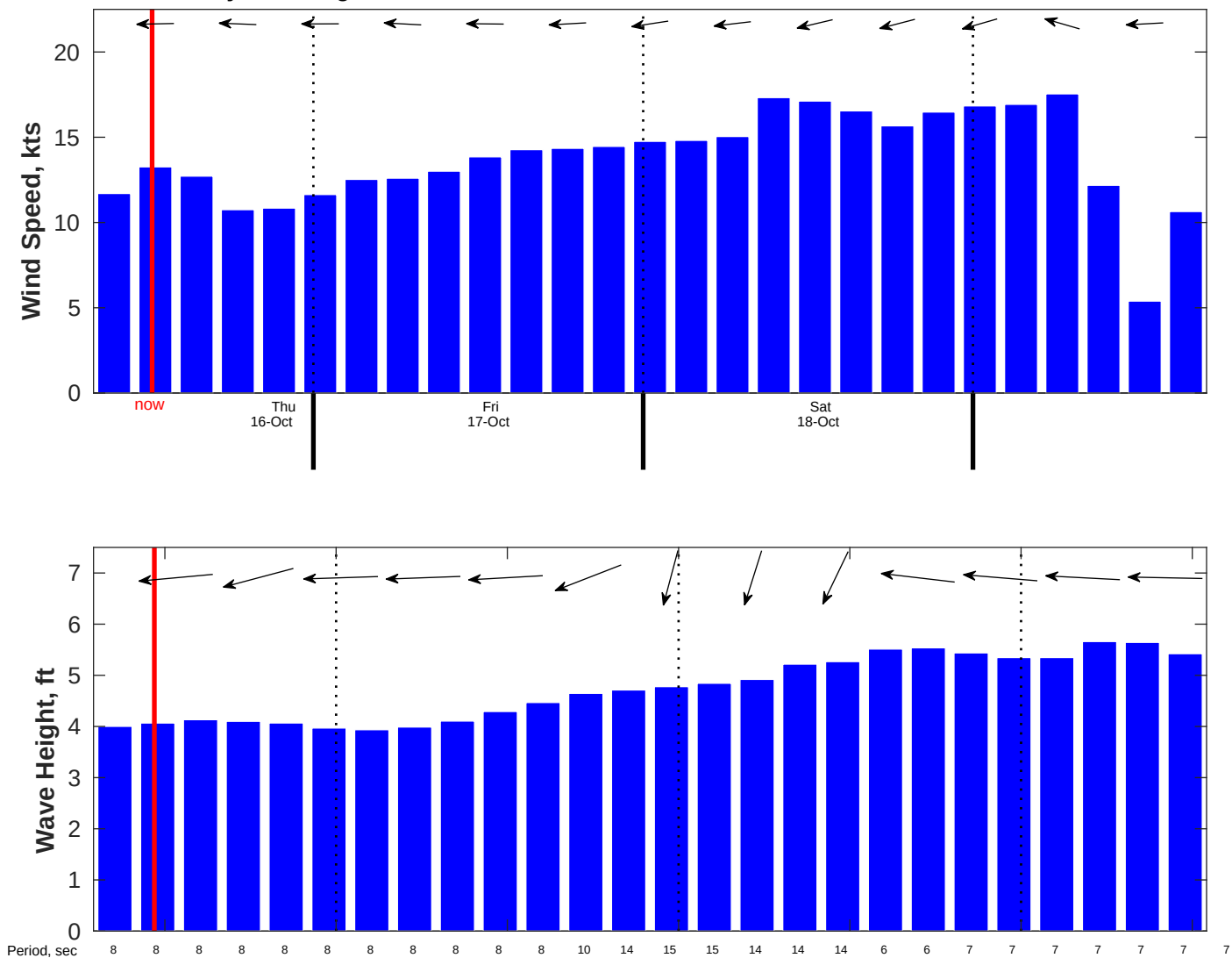
Wind & Wave Forecast for Gyre Passage: Dakar to Trinidad from 16-Oct-2025 07:00:00 to 19-Oct-2025 13:00:00
