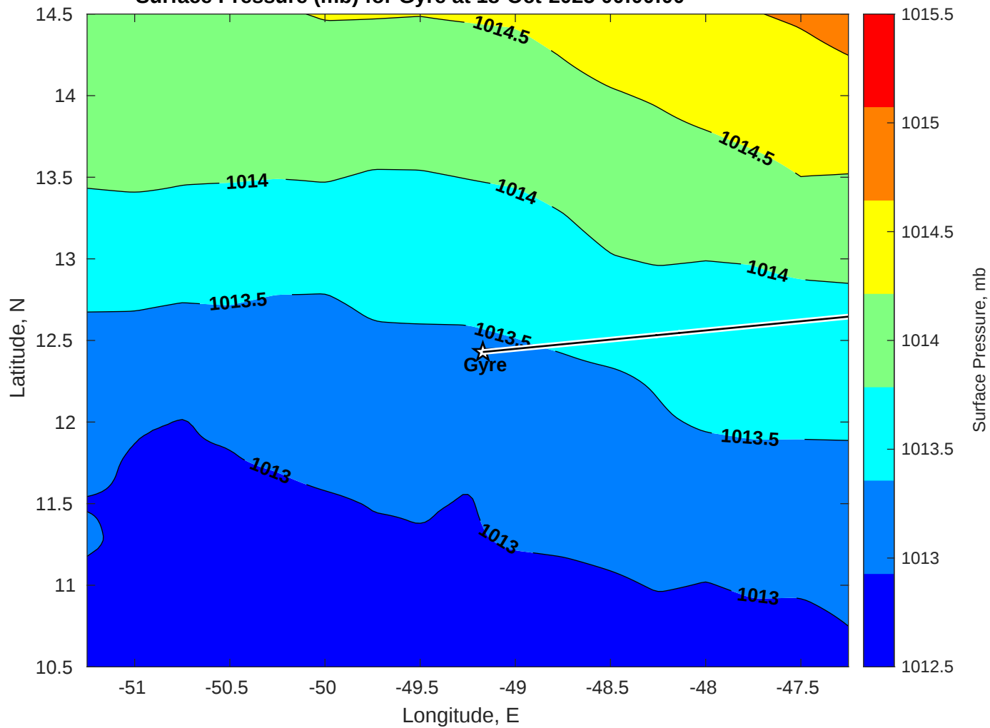
Surface Pressure (mb) for Gyre at 18-Oct-2025 00:00:00
