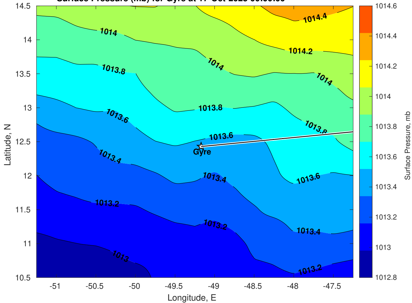
Surface Pressure (mb) for Gyre at 17-Oct-2025 00:00:00
