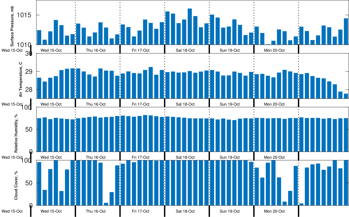
Met Forecast for Gyre from 15-Oct-2025 21:00:00 to 22-Oct-2025 21:00:00
