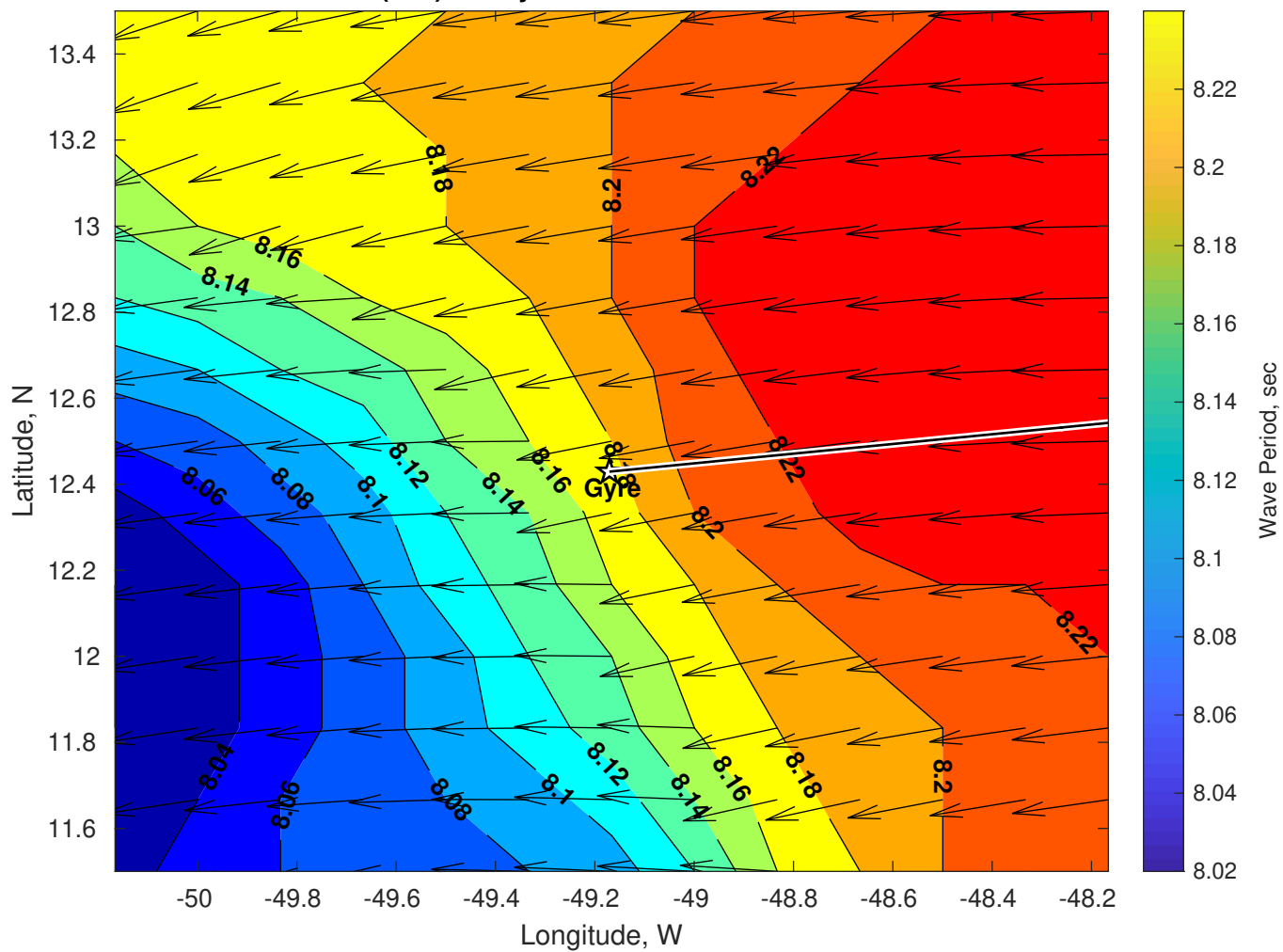
Wave Period (sec) for Gyre at 16-Oct-2025 09:00:00
