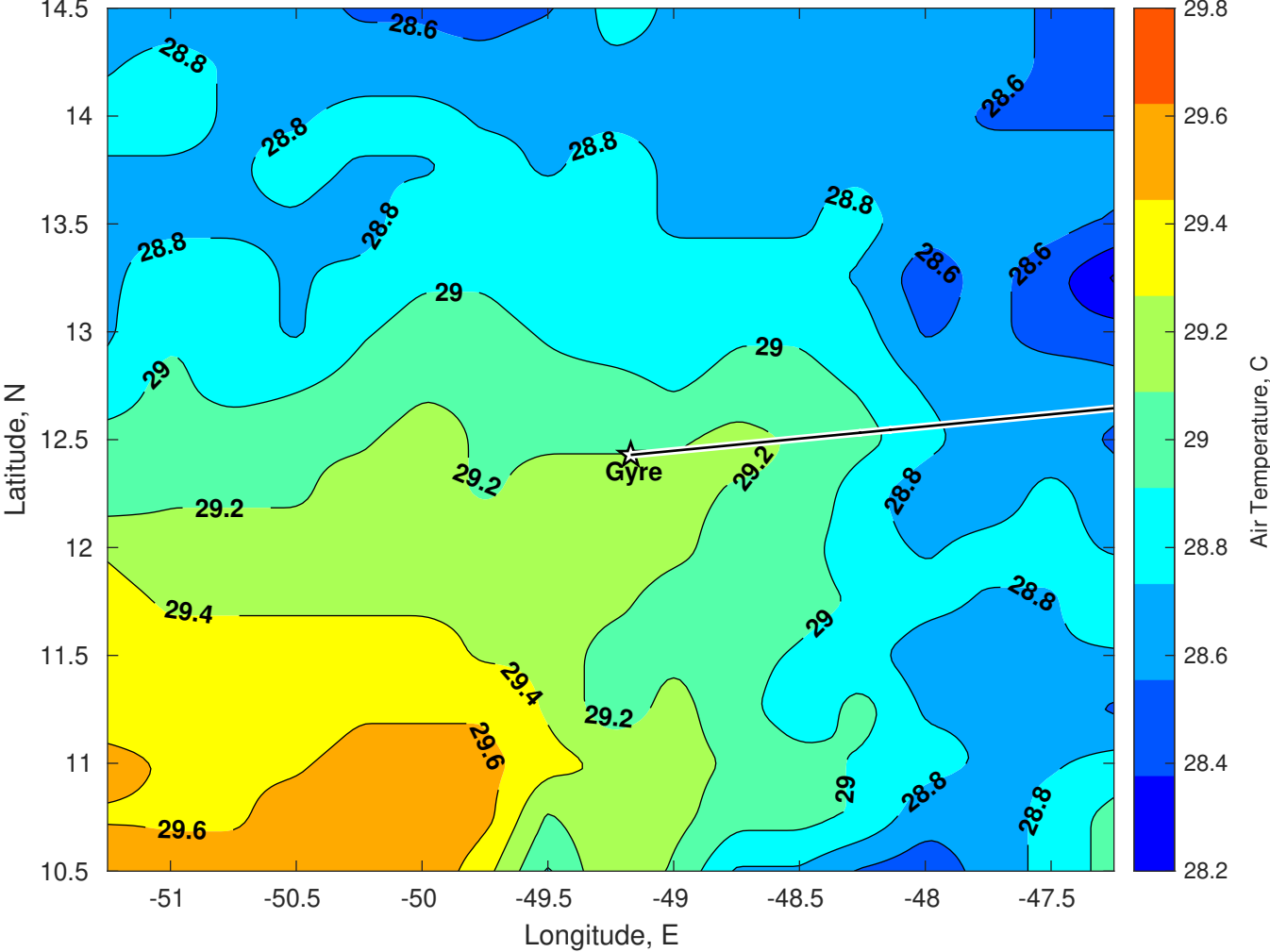
Air Temperature (C) for Gyre at 16-Oct-2025
