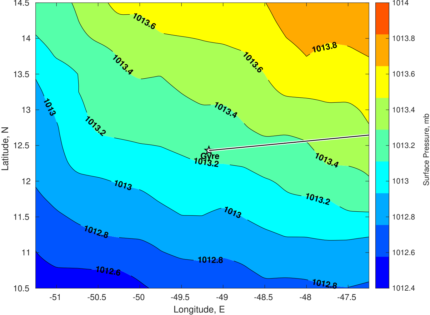
Surface Pressure (mb) for Gyre at 16-Oct-2025 00:00:00
