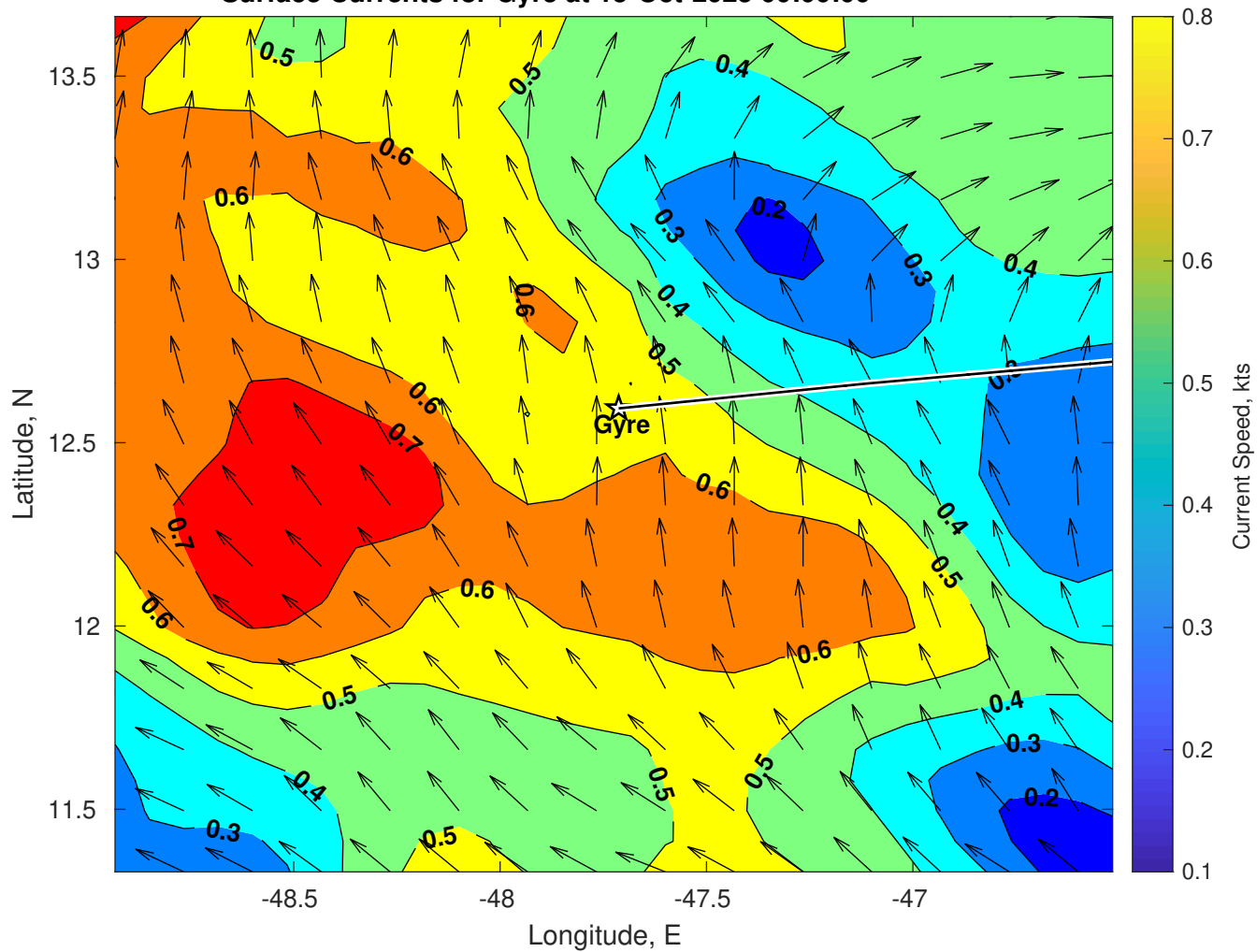
Surface Currents for Gyre at 15-Oct-2025 00:00:00
