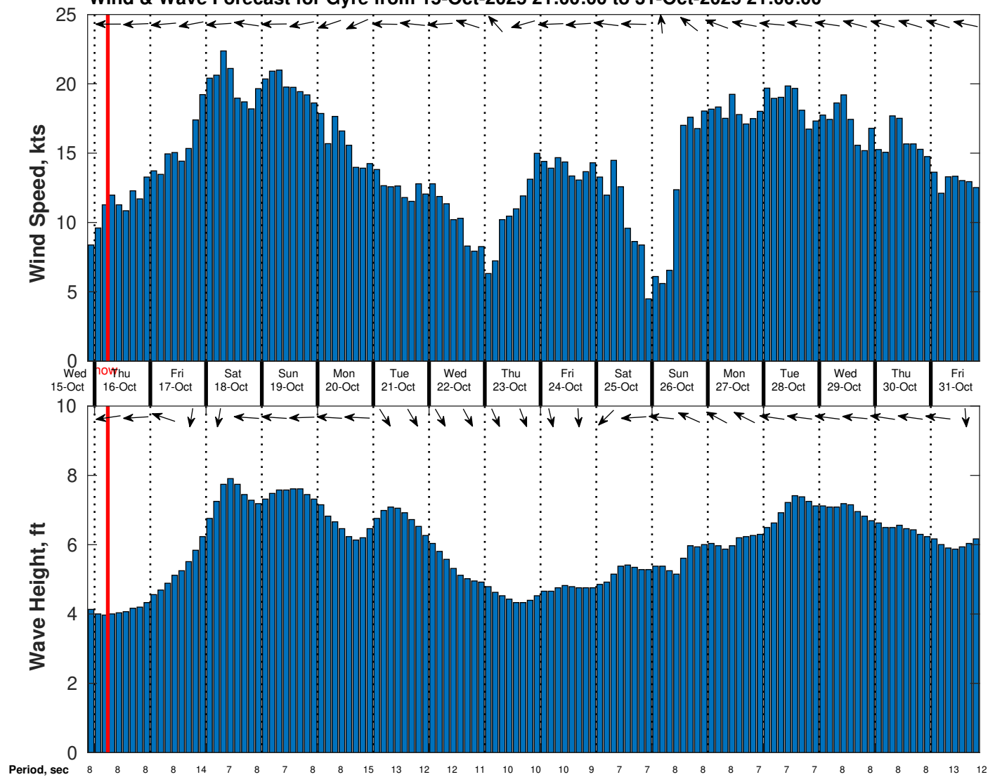
Wind & Wave Forecast for Gyre from 15-Oct-2025 21:00:00 to 31-Oct-2025 21:00:00
