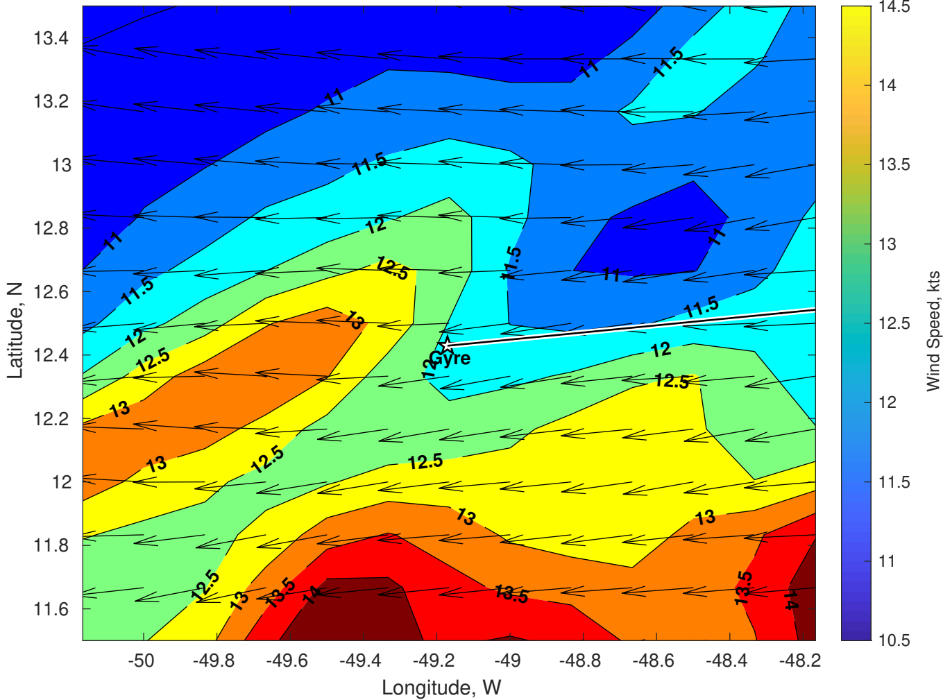
Winds (kts) for Gyre at 16-Oct-2025 09:00:00
