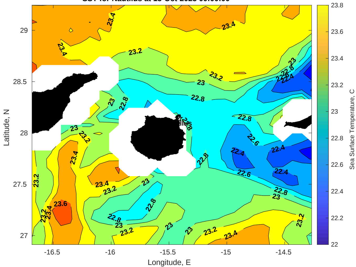
SST for Nautilus at 15-Oct-2025 00:00:00
