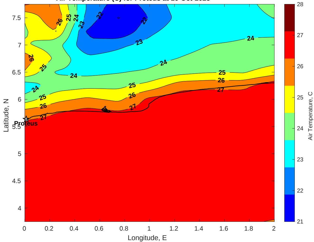
Air Temperature (C) for Proteus at 16-Oct-2025
