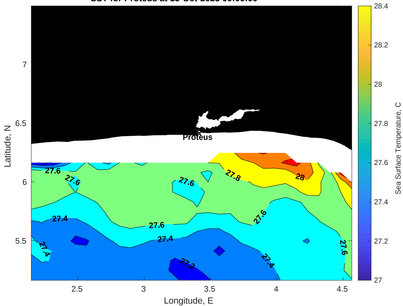
SST for Proteus at 15-Oct-2025 00:00:00
