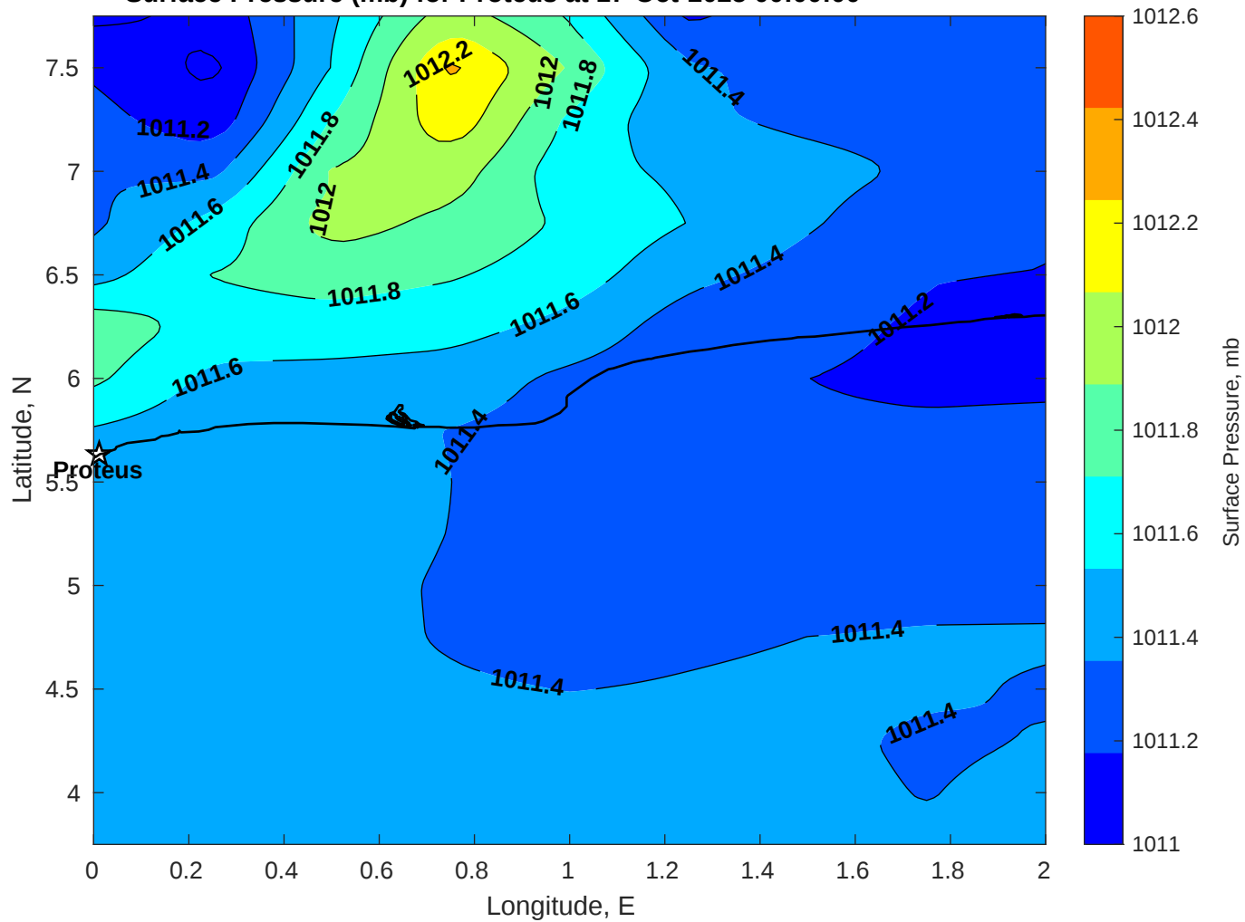
Surface Pressure (mb) for Proteus at 17-Oct-2025 00:00:00
