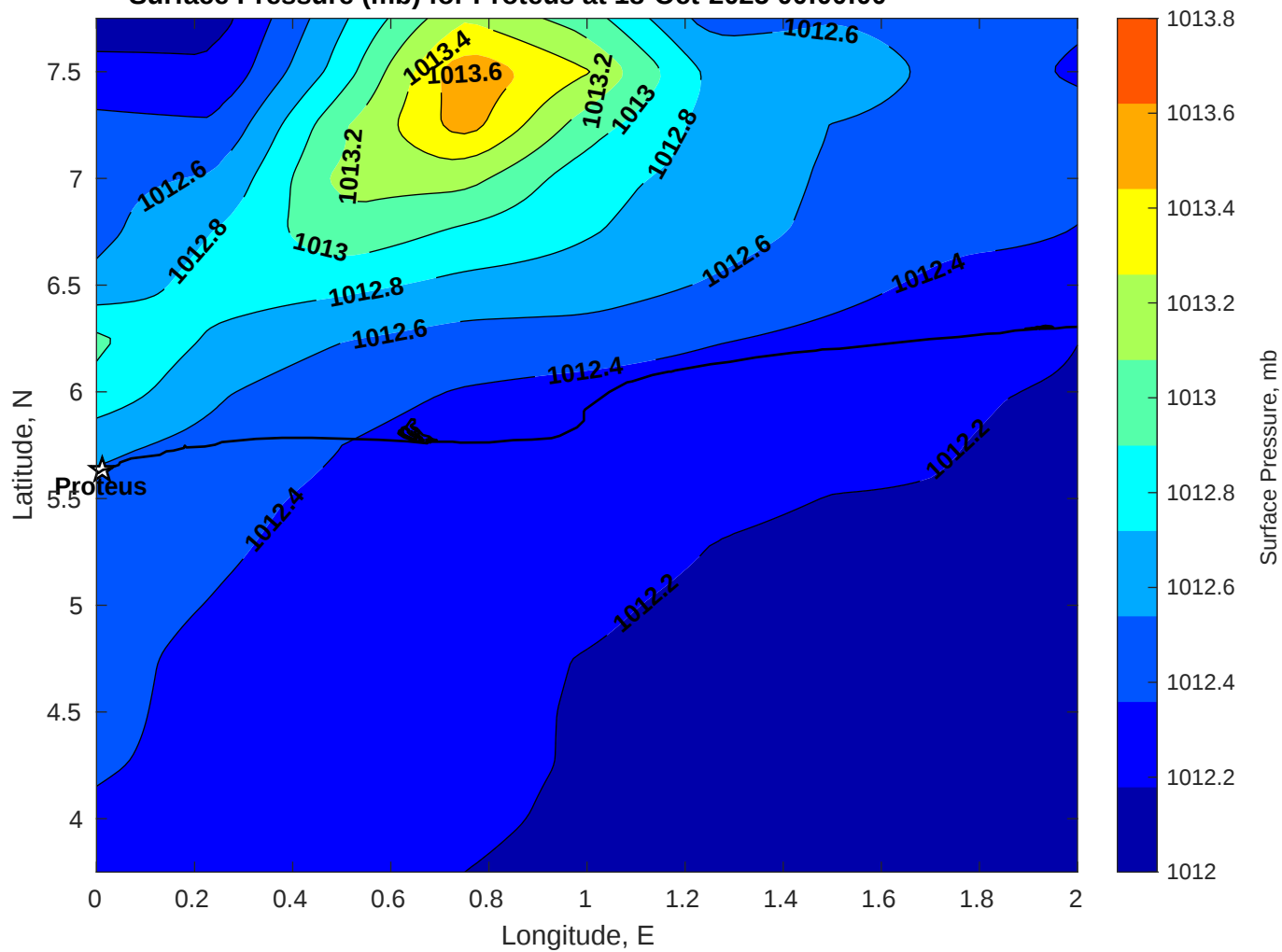
Surface Pressure (mb) for Proteus at 18-Oct-2025 00:00:00
