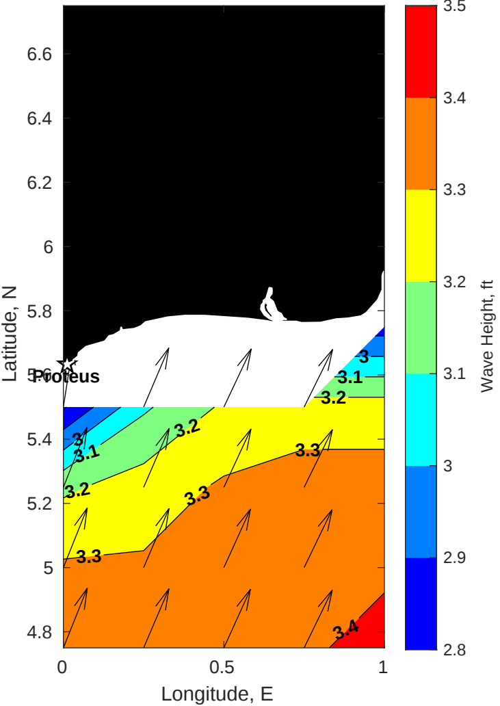
Wave Height (ft) for Proteus at 16-Oct-2025 09:00:00
