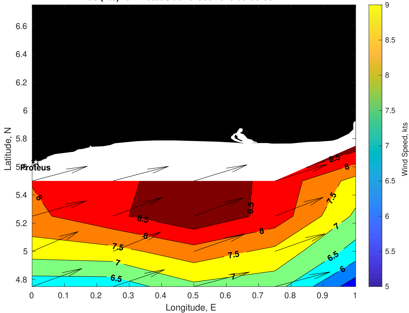
Winds (kts) for Proteus at 16-Oct-2025 09:00:00
