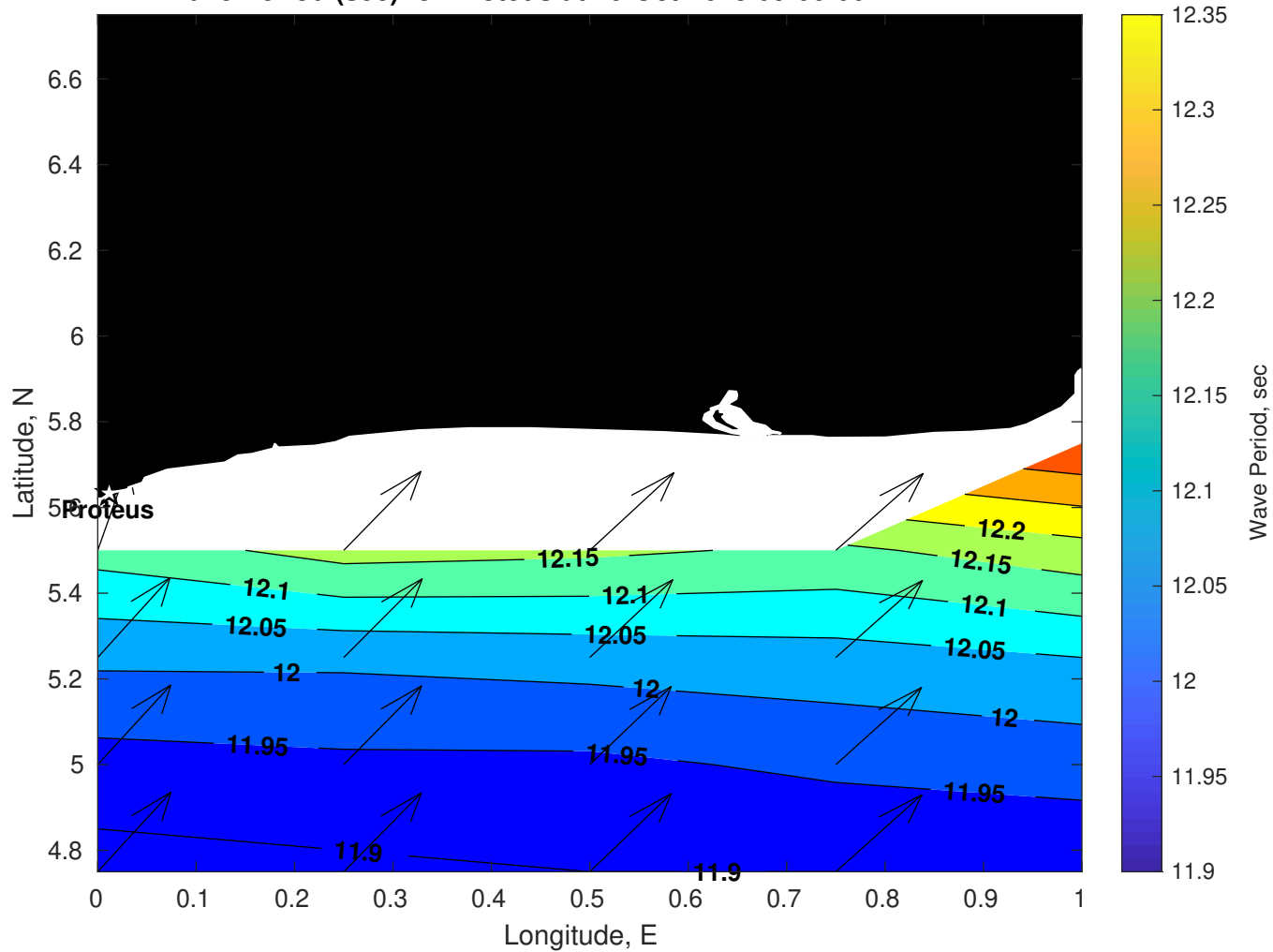
Wave Period (sec) for Proteus at 16-Oct-2025 09:00:00
