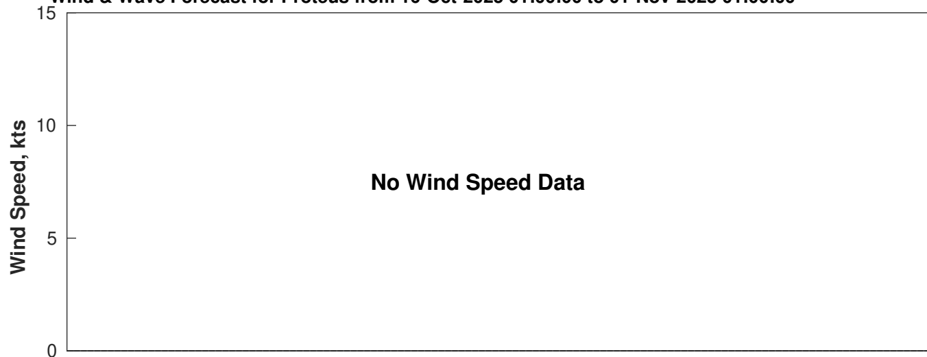
Wind & Wave Forecast for Proteus from 16-Oct-2025 01:00:00 to 01-Nov-2025 01:00:00
