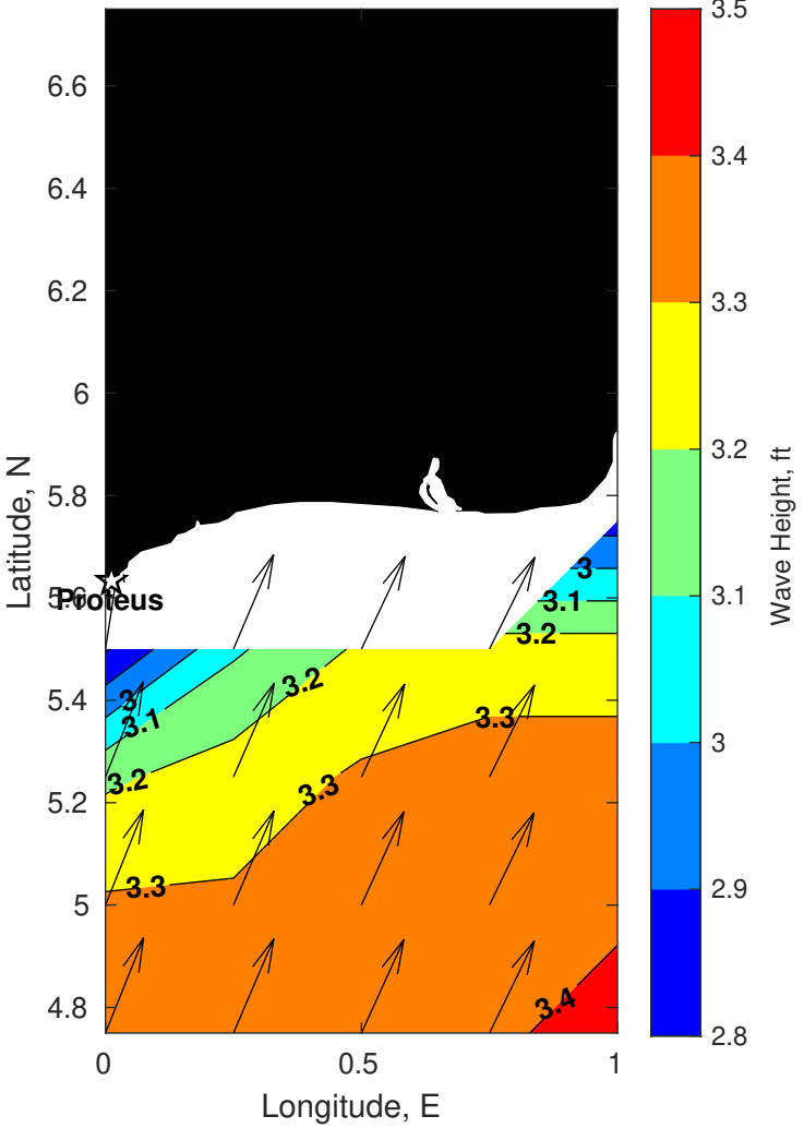
Wave Height (ft) for Proteus at 16-Oct-2025 09:00:00
