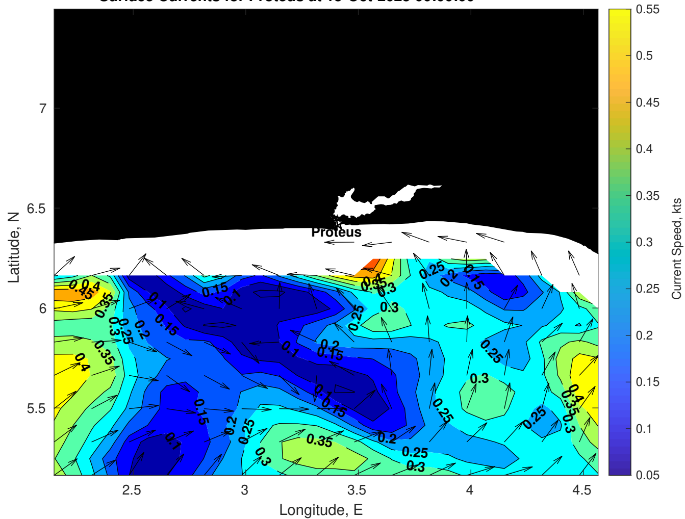
Surface Currents for Proteus at 15-Oct-2025 00:00:00
