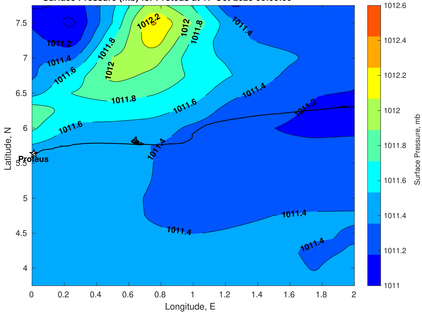
Surface Pressure (mb) for Proteus at 17-Oct-2025 00:00:00
