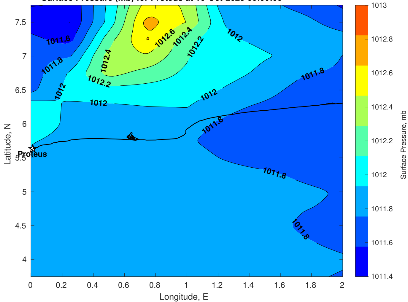
Surface Pressure (mb) for Proteus at 16-Oct-2025 00:00:00
