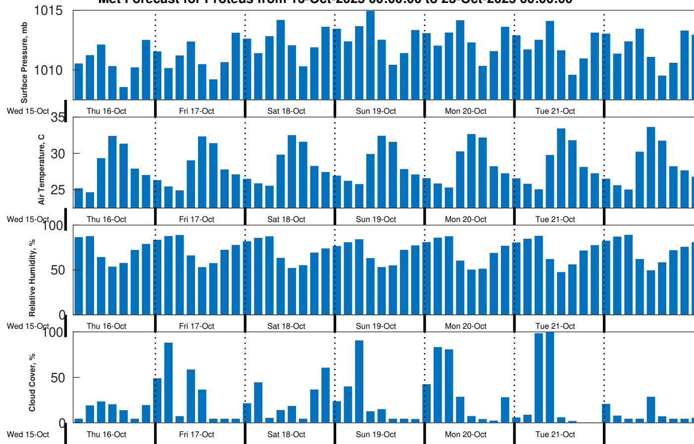
Met Forecast for Proteus from 16-Oct-2025 00:00:00 to 23-Oct-2025 00:00:00
