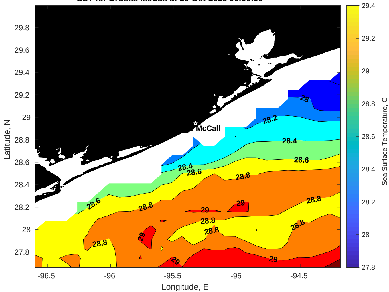
SST for Brooks McCall at 16-Oct-2025 00:00:00
