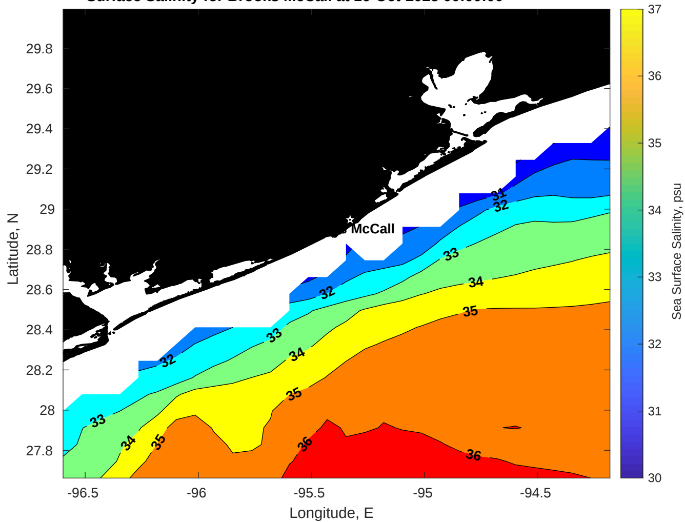
Surface Salinity for Brooks McCall at 16-Oct-2025 00:00:00
