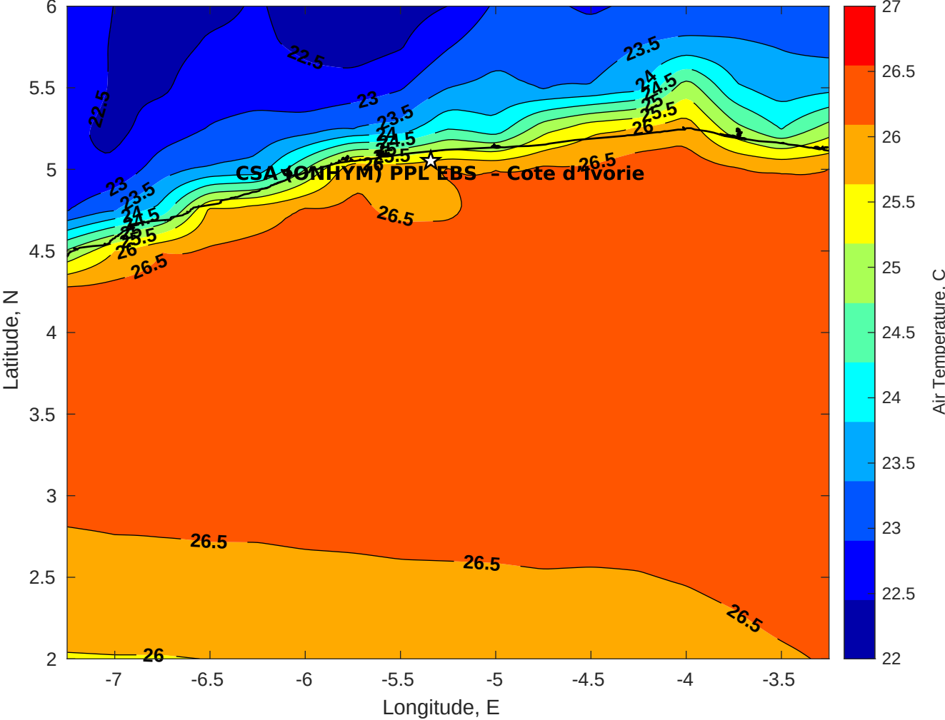
Air Temperature (C) for CSA (ONHYM) PPL EBS - Cote d'Ivoire at 17-Oct-2025
