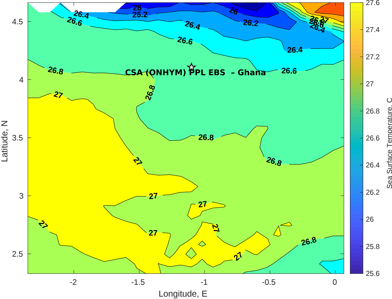
SST for CSA (ONHYM) PPL EBS - Ghana at 16-Oct-2025 00:00:00
