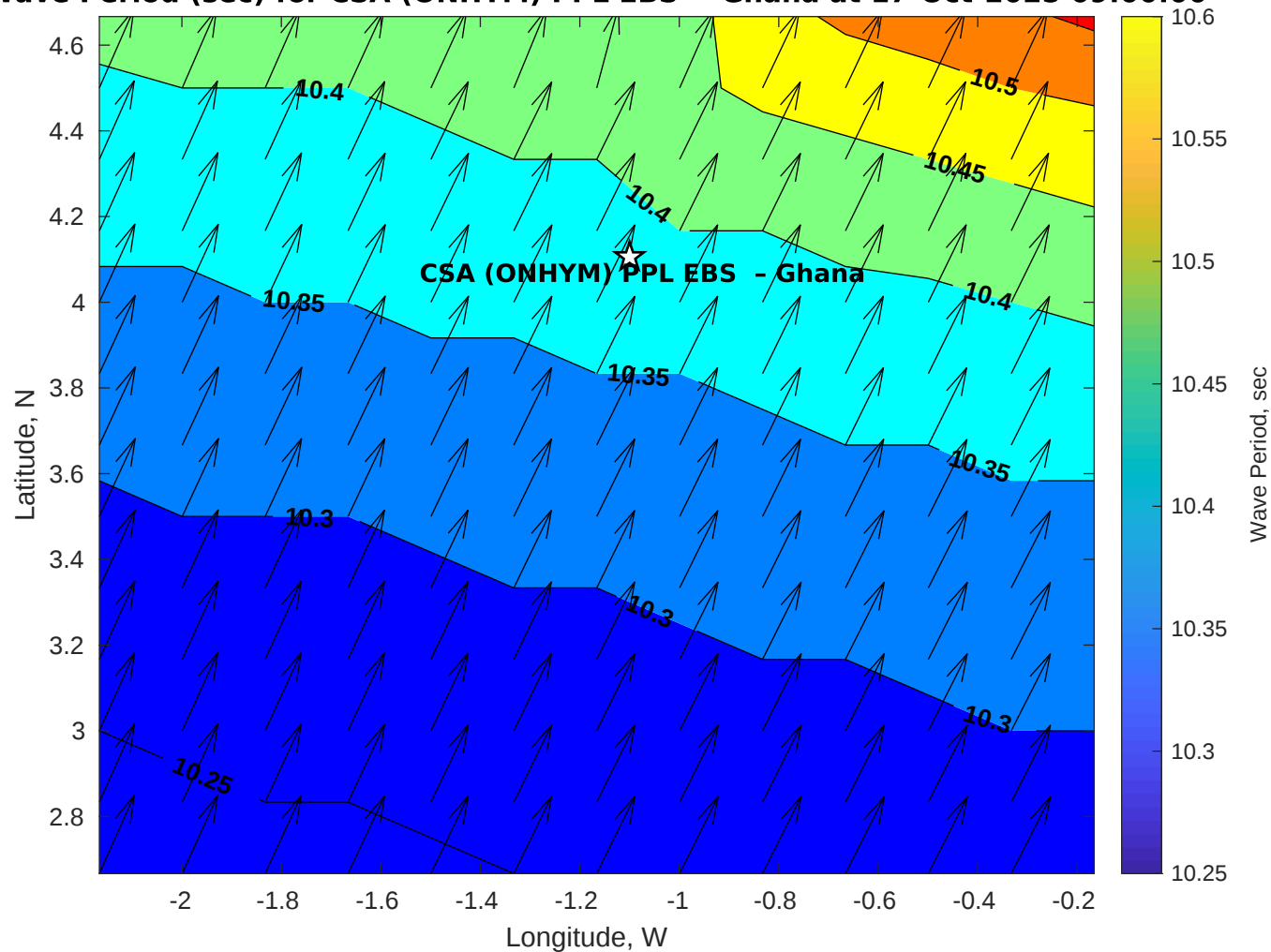
Wave Period (sec) for CSA (ONHYM) PPL EBS - Ghana at 17-Oct-2025 09:00:00
