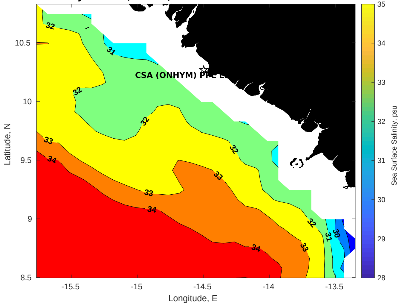
Surface Salinity for CSA (ONHYM) PPL EBS - Guinea at 16-Oct-2025 00:00:00
