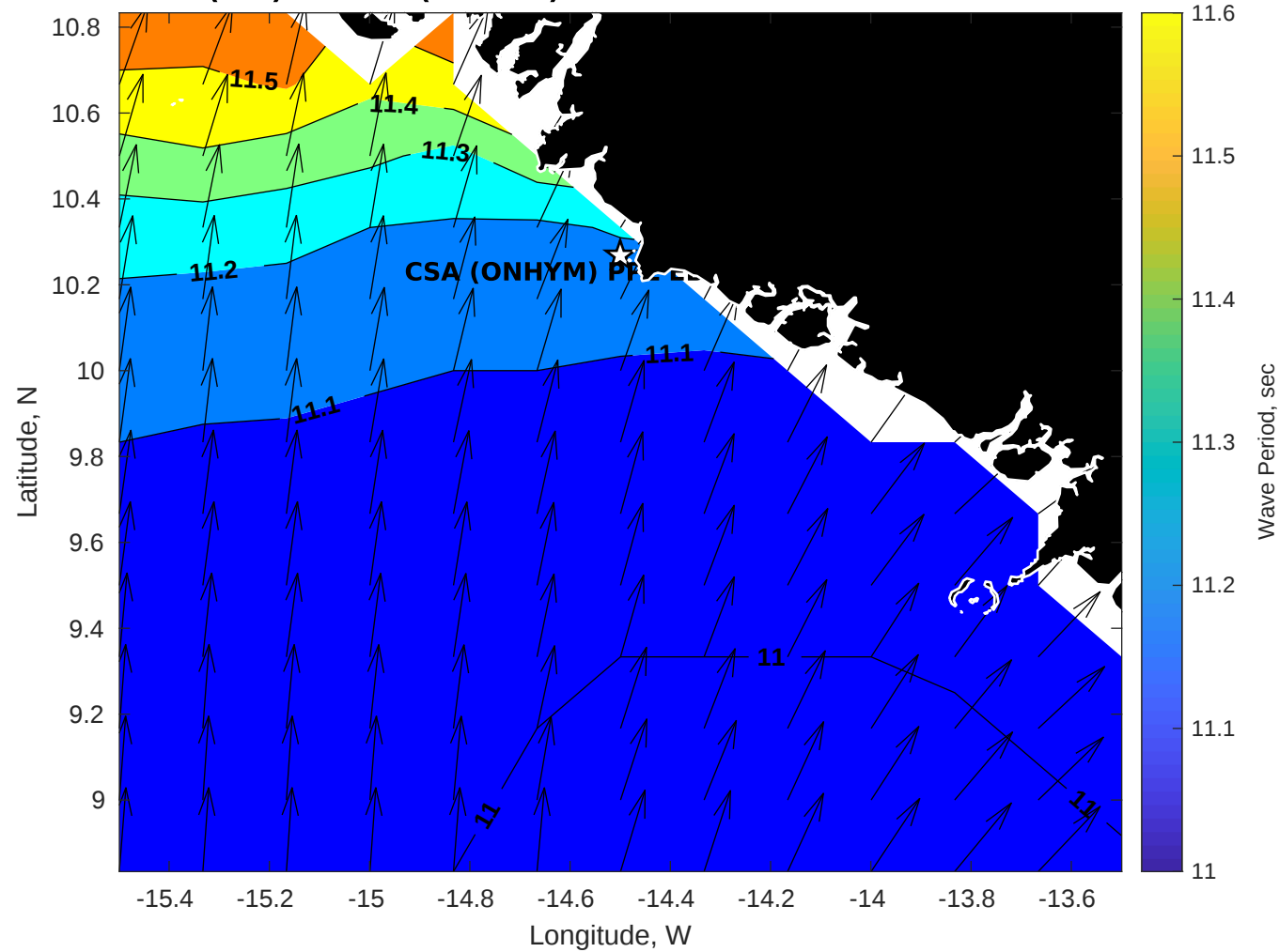
Wave Period (sec) for CSA (ONHYM) PPL EBS - Guinea at 17-Oct-2025 09:00:00
