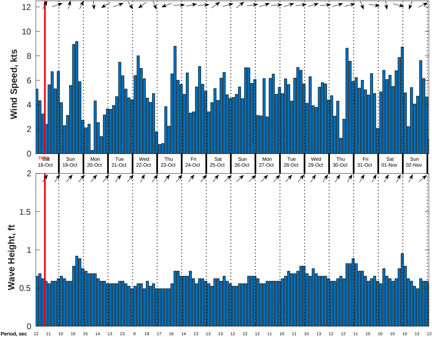
Wind & Wave Forecast for CSA (ONHYM) PPL EBS - Guinea from 17-Oct-2025 01:00:00 to 02-Nov-2025 01:00:00
