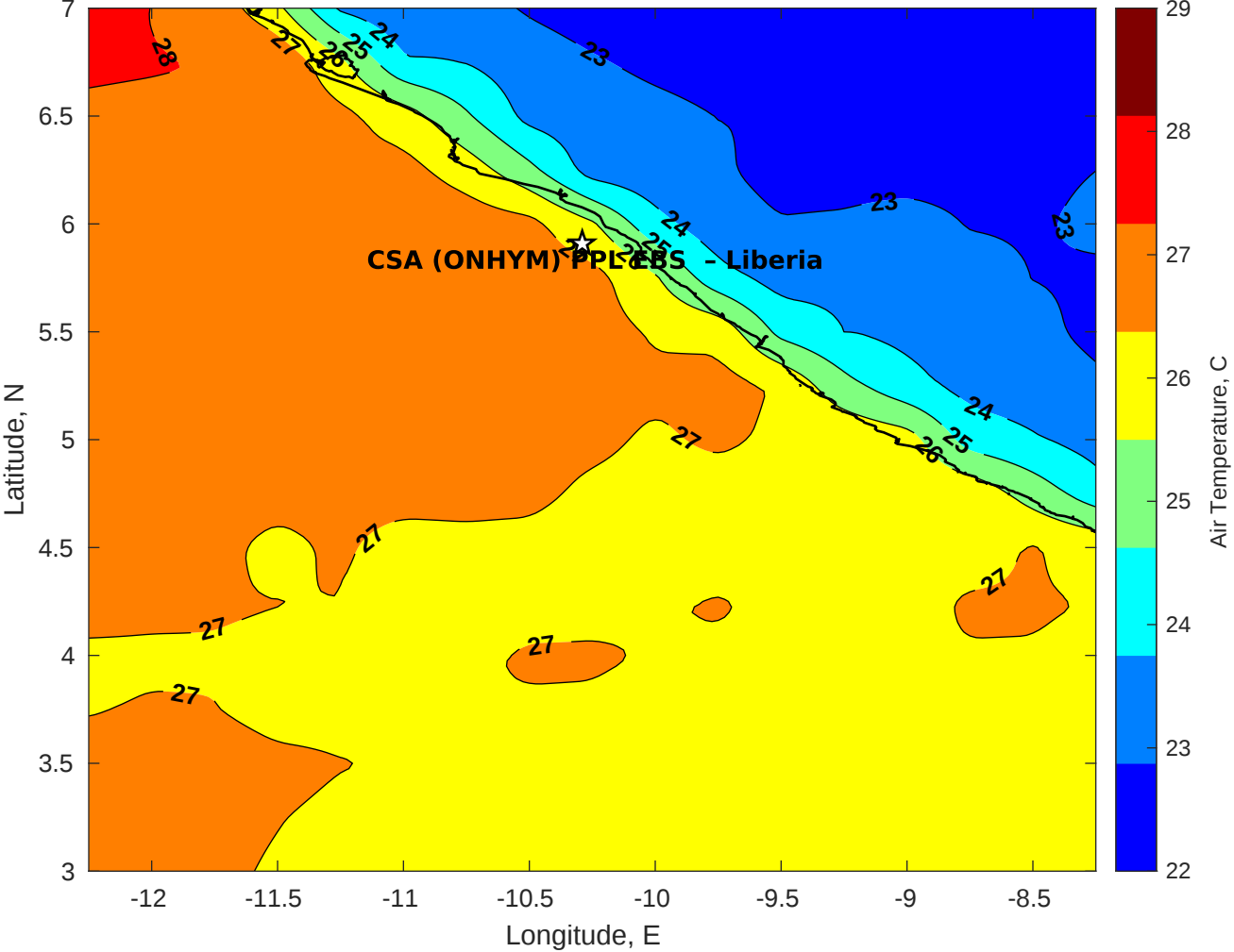
Air Temperature (C) for CSA (ONHYM) PPL EBS - Liberia at 17-Oct-2025
