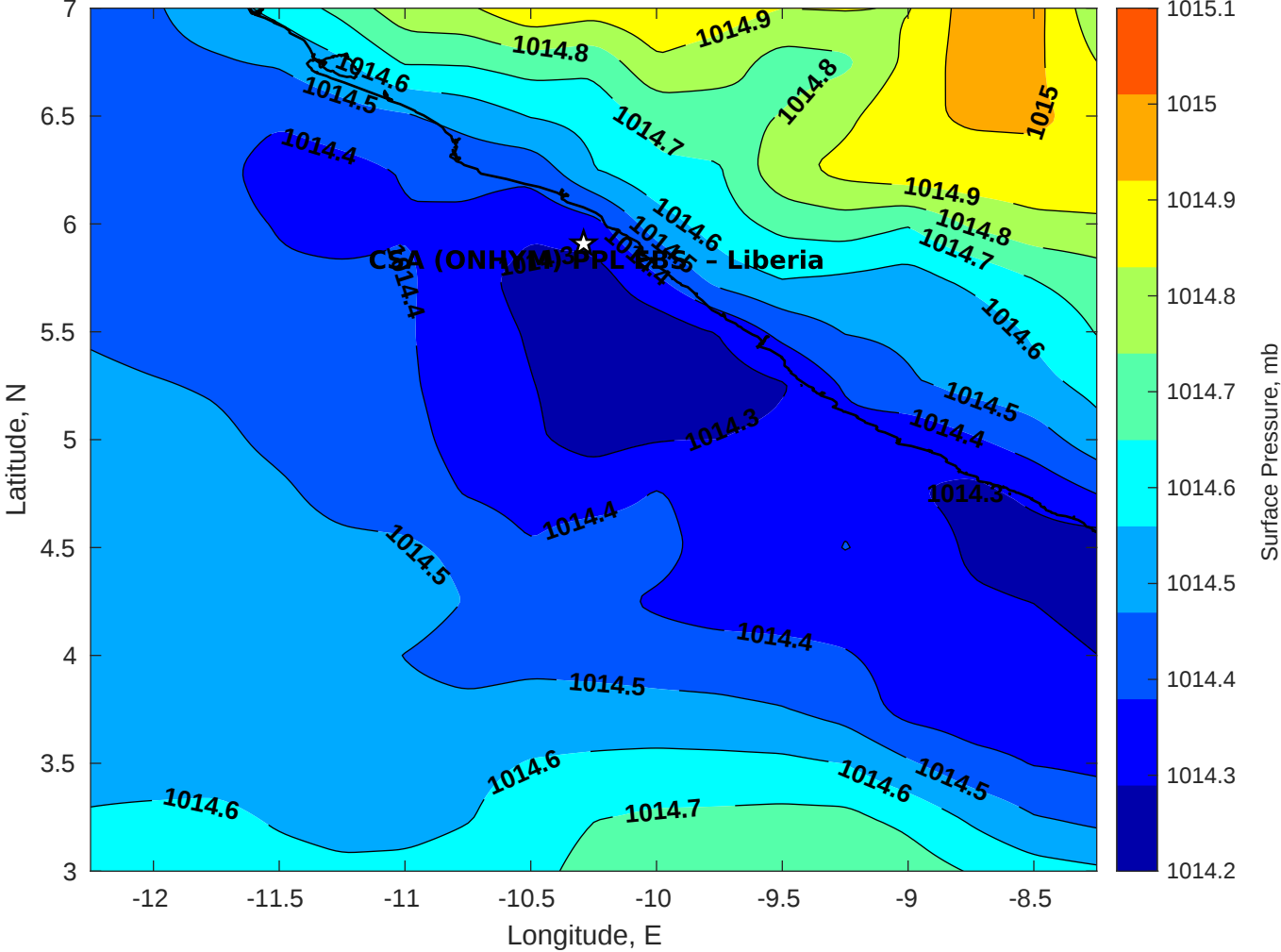
Surface Pressure (mb) for CSA (ONHYM) PPL EBS - Liberia at 19-Oct-2025 00:00:00
