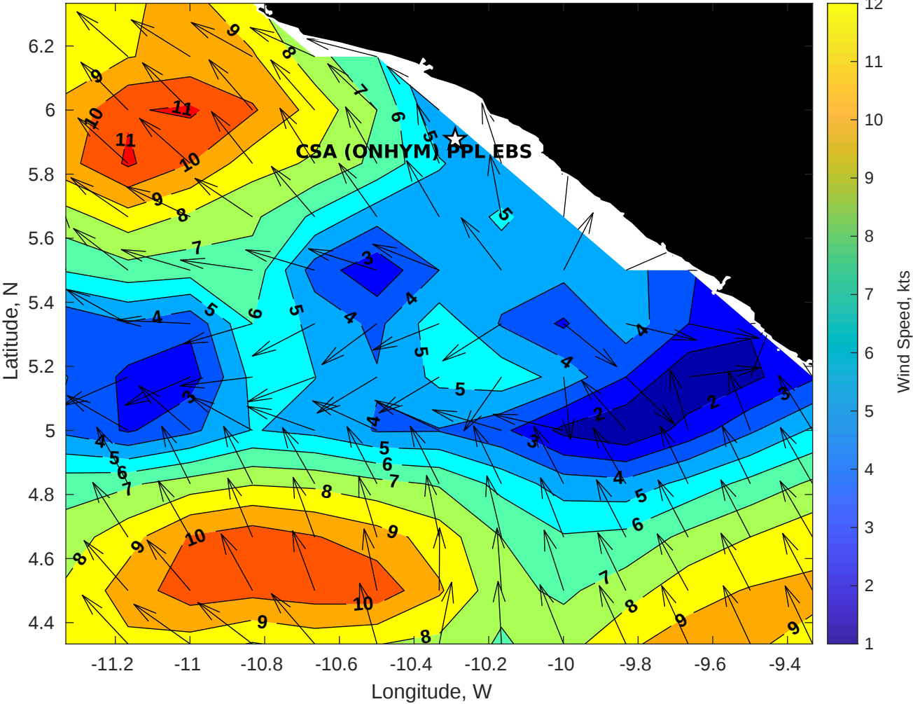
Winds (kts) for CSA (ONHYM) PPL EBS - Liberia at 17-Oct-2025 09:00:00
