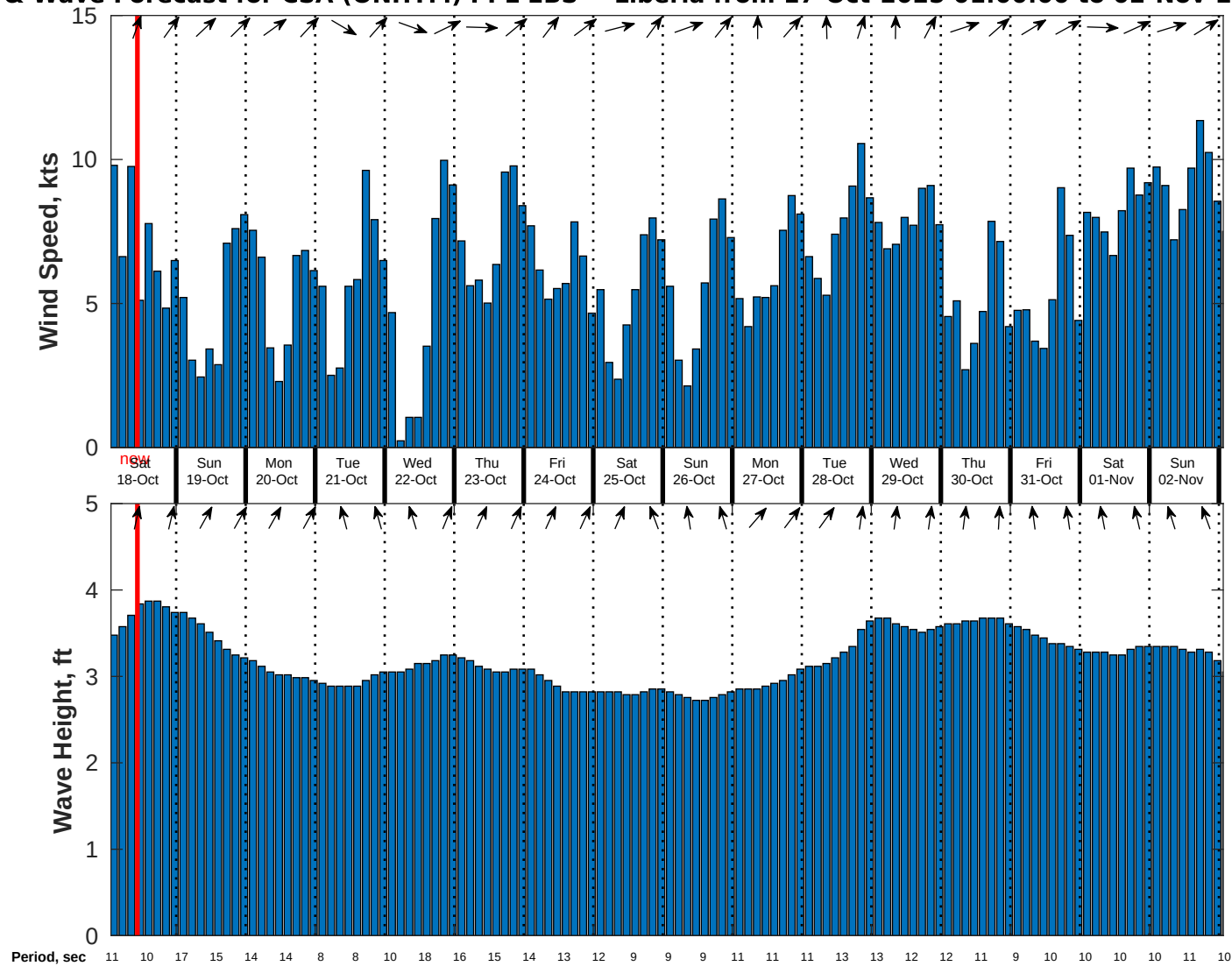
Wind & Wave Forecast for CSA (ONHYM) PPL EBS - Liberia from 17-Oct-2025 01:00:00 to 02-Nov-2025 01:00:00
