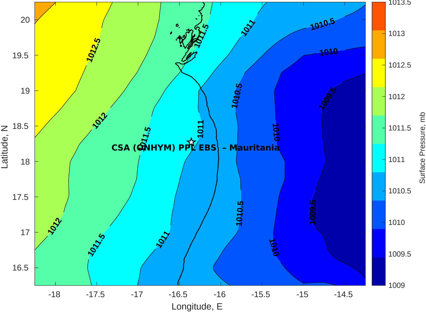
Surface Pressure (mb) for CSA (ONHYM) PPL EBS - Mauritania at 18-Oct-2025 00:00:00
