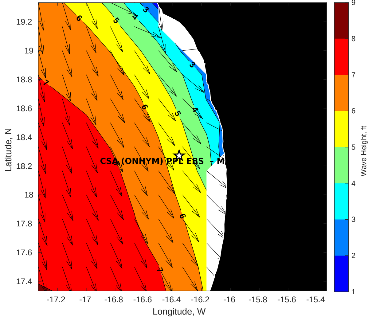
Wave Height (ft) for CSA (ONHYM) PPL EBS - Mauritania at 17-Oct-2025 09:00:00
