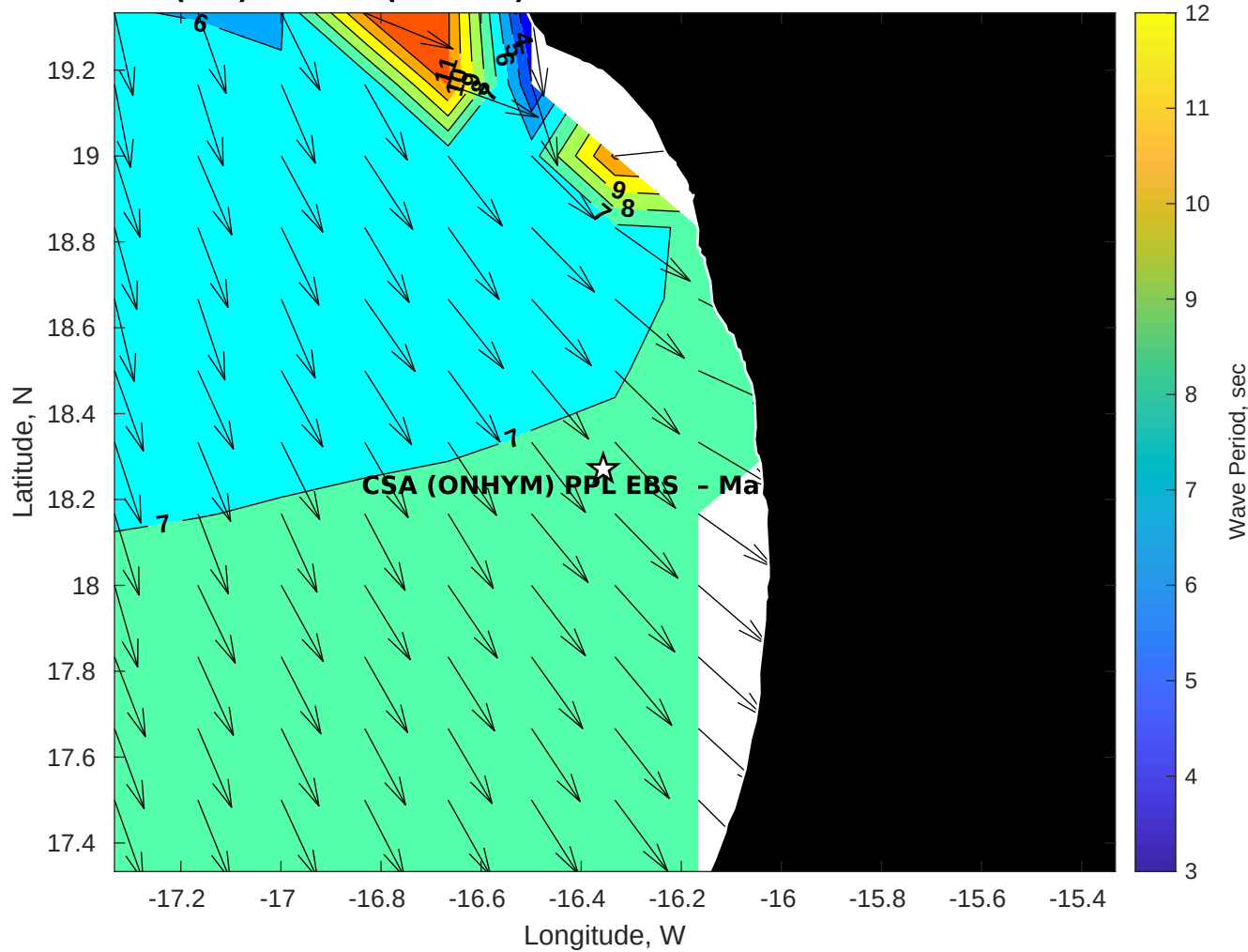
Wave Period (sec) for CSA (ONHYM) PPL EBS - Mauritania at 17-Oct-2025 09:00:00
