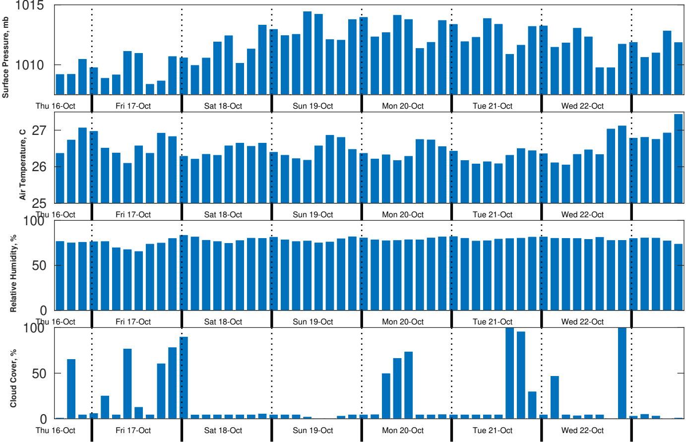
Met Forecast for CSA (ONHYM) PPL EBS - Mauritania from 16-Oct-2025 12:00:00 to 23-Oct-2025 12:00:00
