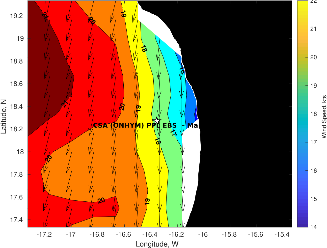
Winds (kts) for CSA (ONHYM) PPL EBS - Mauritania at 17-Oct-2025 09:00:00
