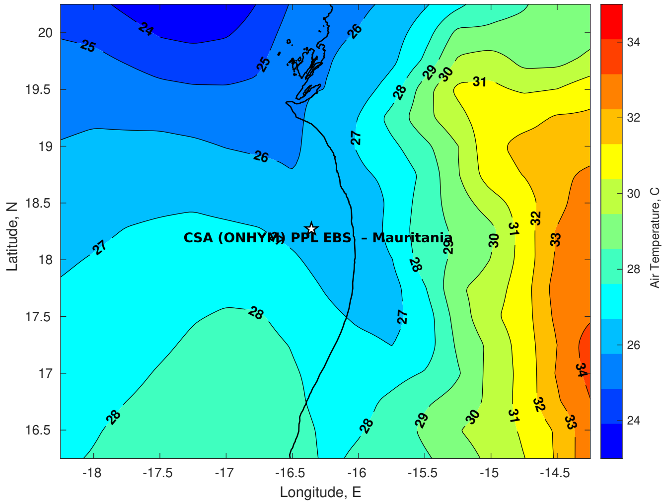
Air Temperature (C) for CSA (ONHYM) PPL EBS - Mauritania at 17-Oct-2025
