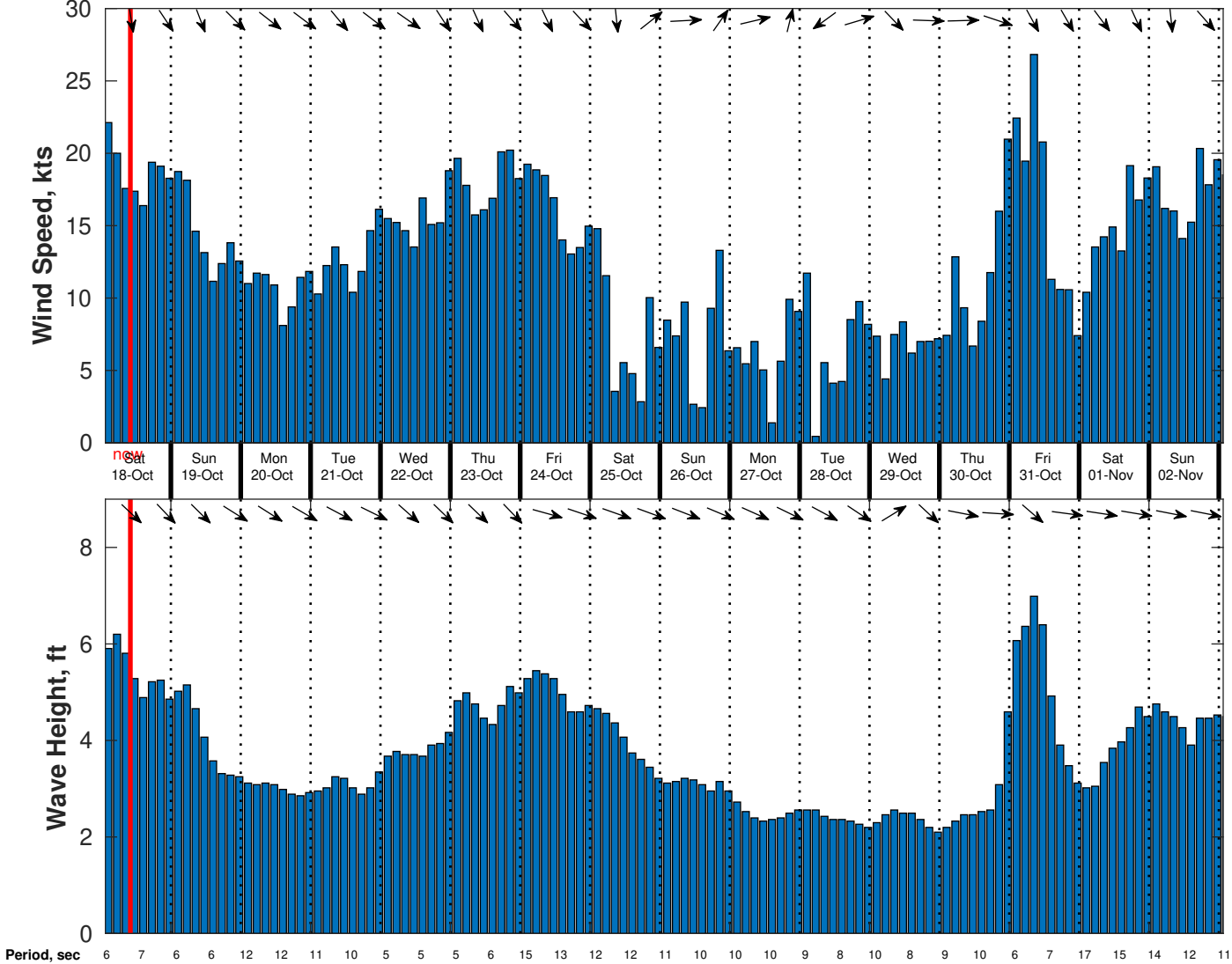
Wind & Wave Forecast for CSA (ONHYM) PPL EBS - Mauritania from 17-Oct-2025 01:00:00 to 02-Nov-2025 01:00:00
