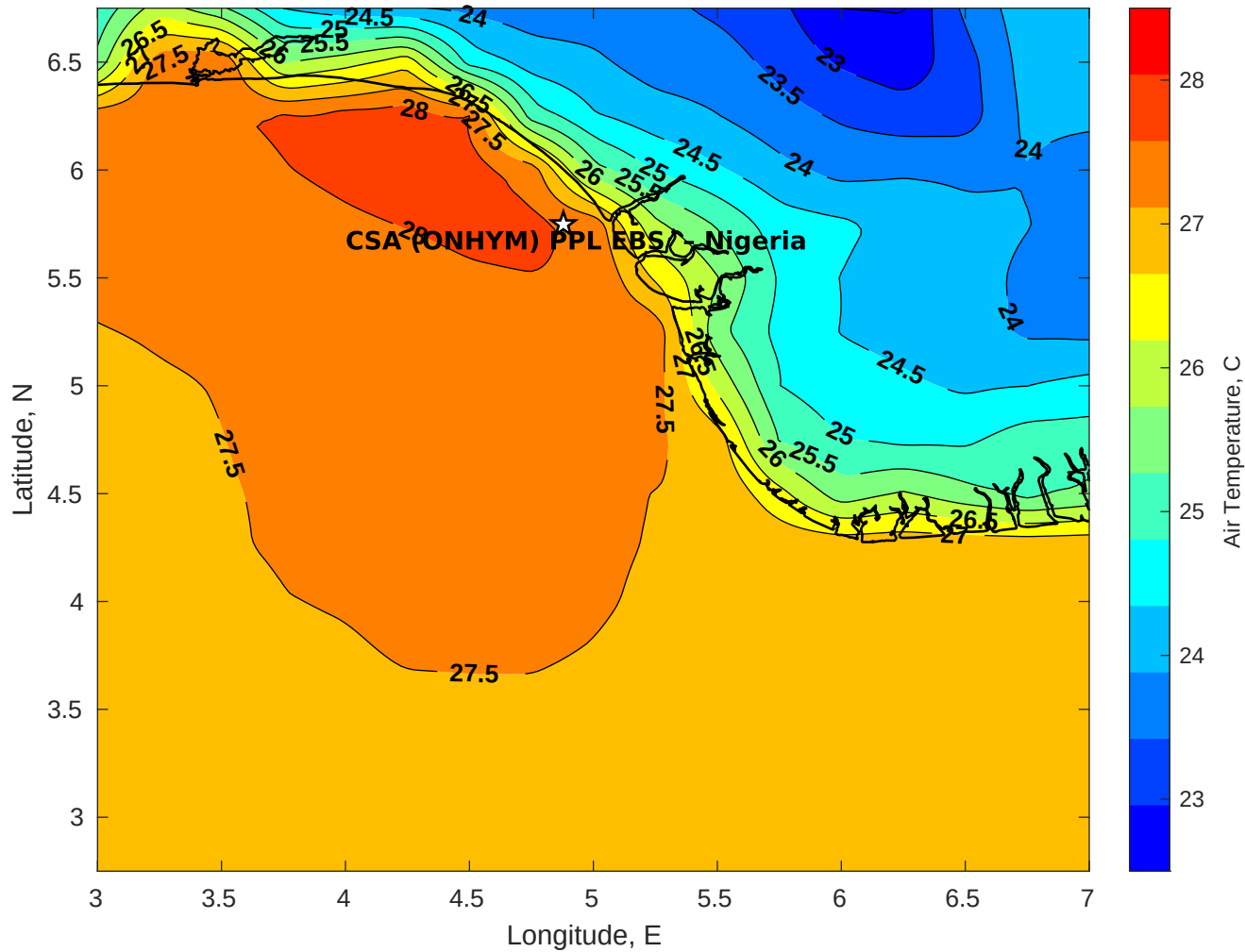
Air Temperature (C) for CSA (ONHYM) PPL EBS - Nigeria at 17-Oct-2025
