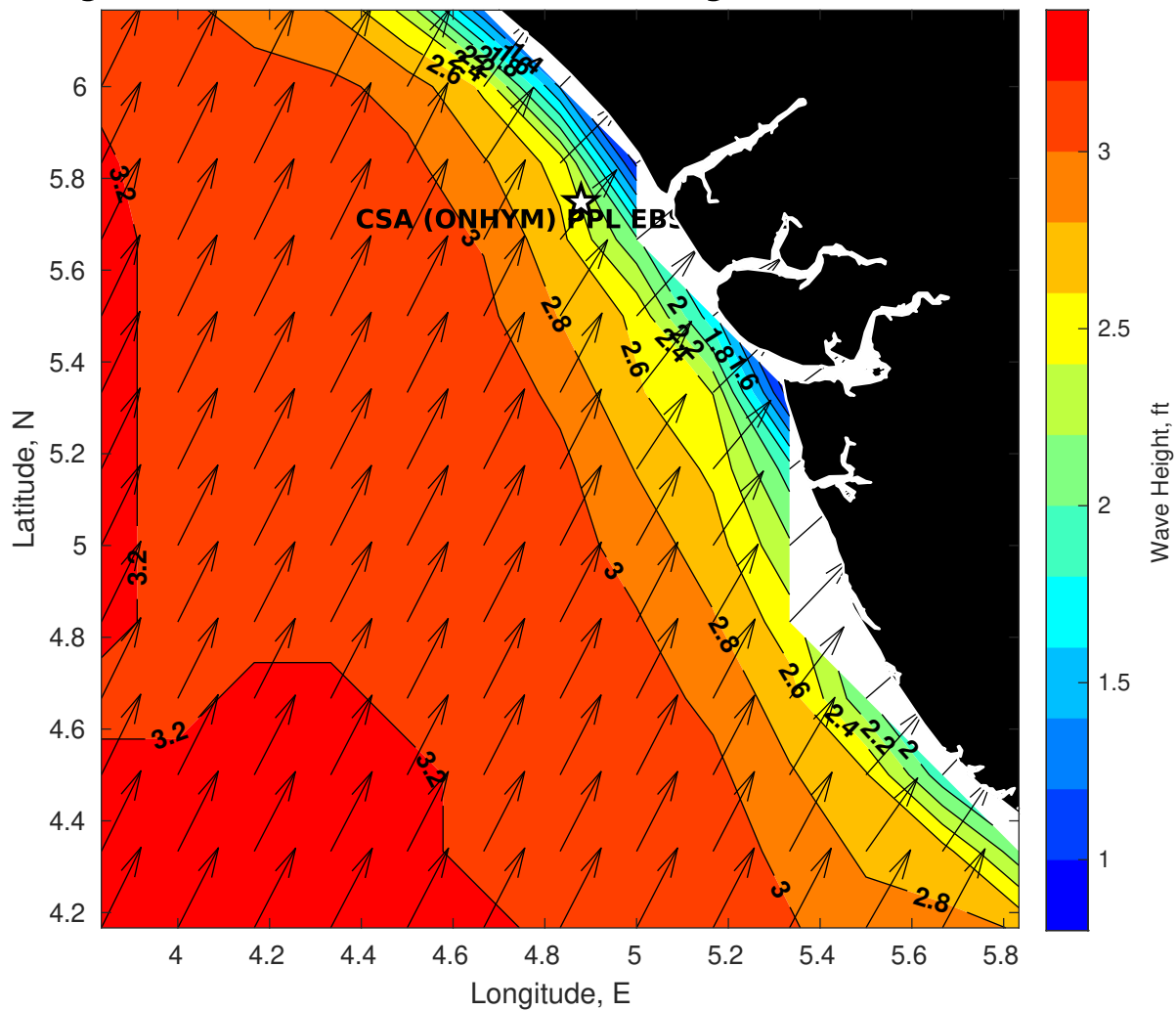
Wave Height (ft) for CSA (ONHYM) PPL EBS - Nigeria at 17-Oct-2025 09:00:00
