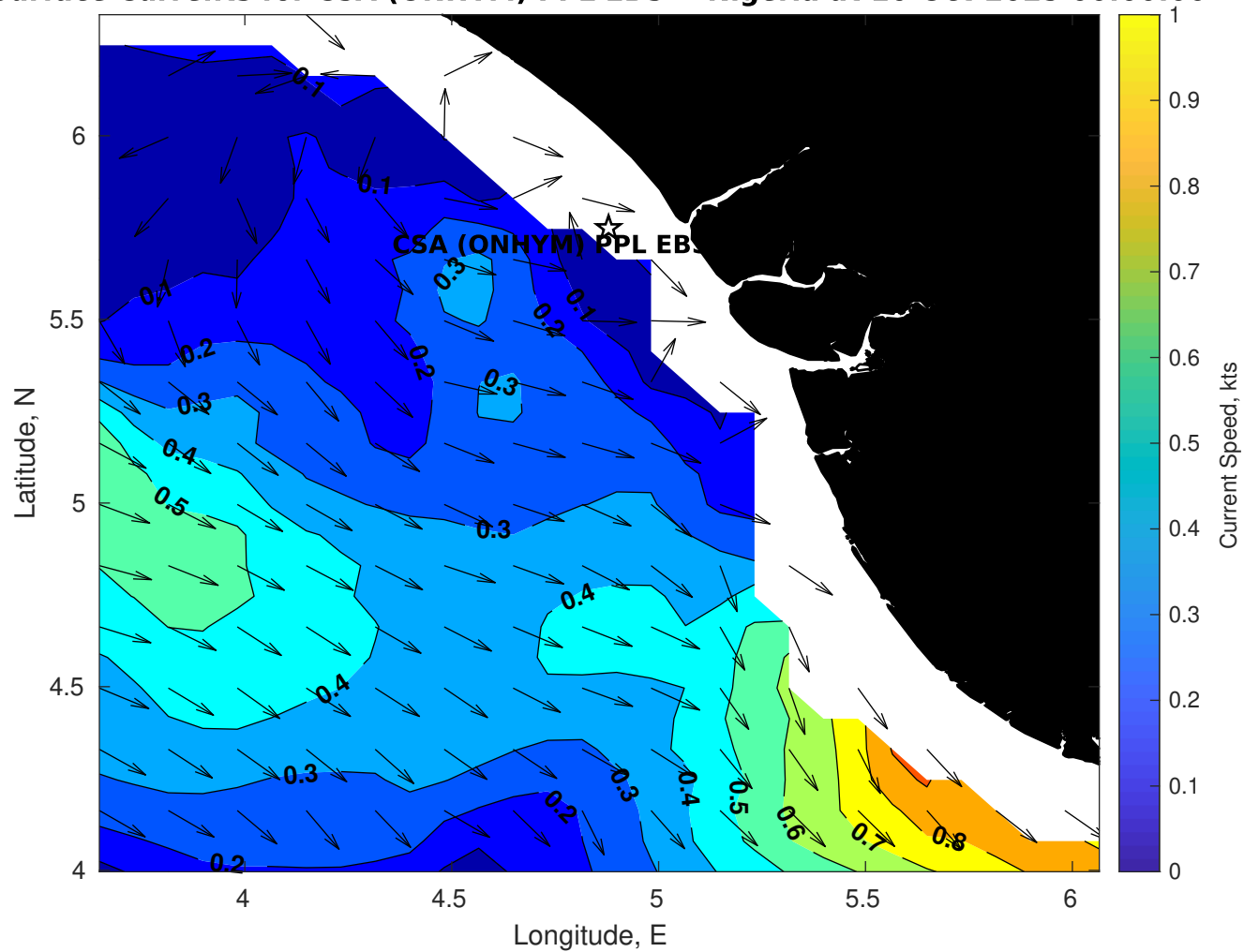
Surface Currents for CSA (ONHYM) PPL EBS - Nigeria at 16-Oct-2025 00:00:00
