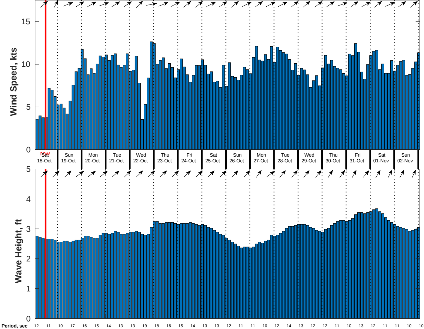
Wind & Wave Forecast for CSA (ONHYM) PPL EBS - Nigeria from 17-Oct-2025 02:00:00 to 02-Nov-2025 02:00:00
