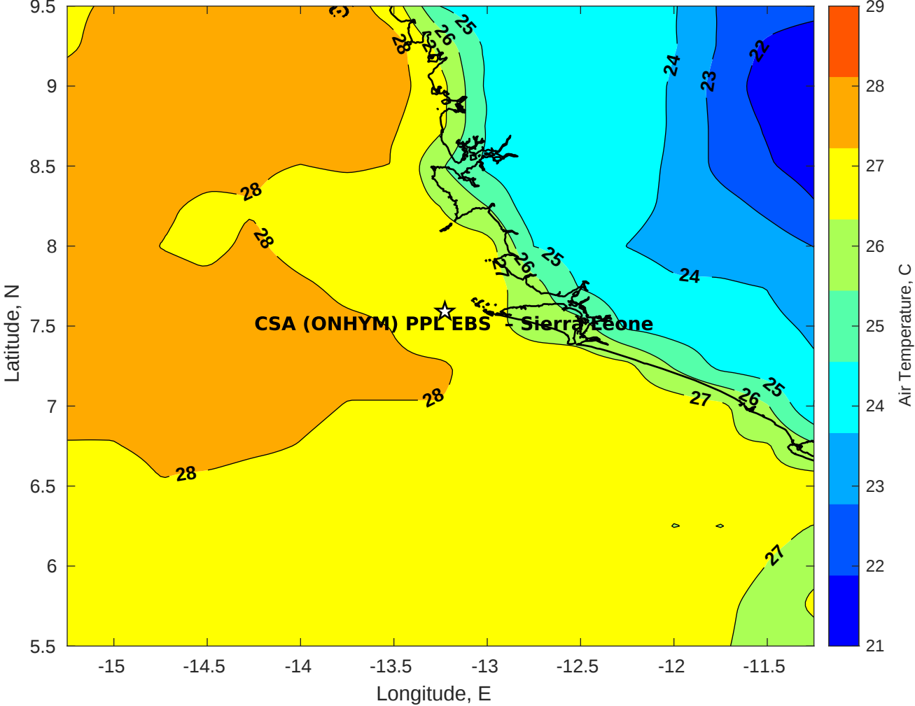
Air Temperature (C) for CSA (ONHYM) PPL EBS - Sierra Leone at 17-Oct-2025
