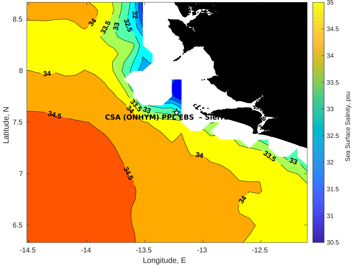
Surface Salinity for CSA (ONHYM) PPL EBS - Sierra Leone at 16-Oct-2025 00:00:00
