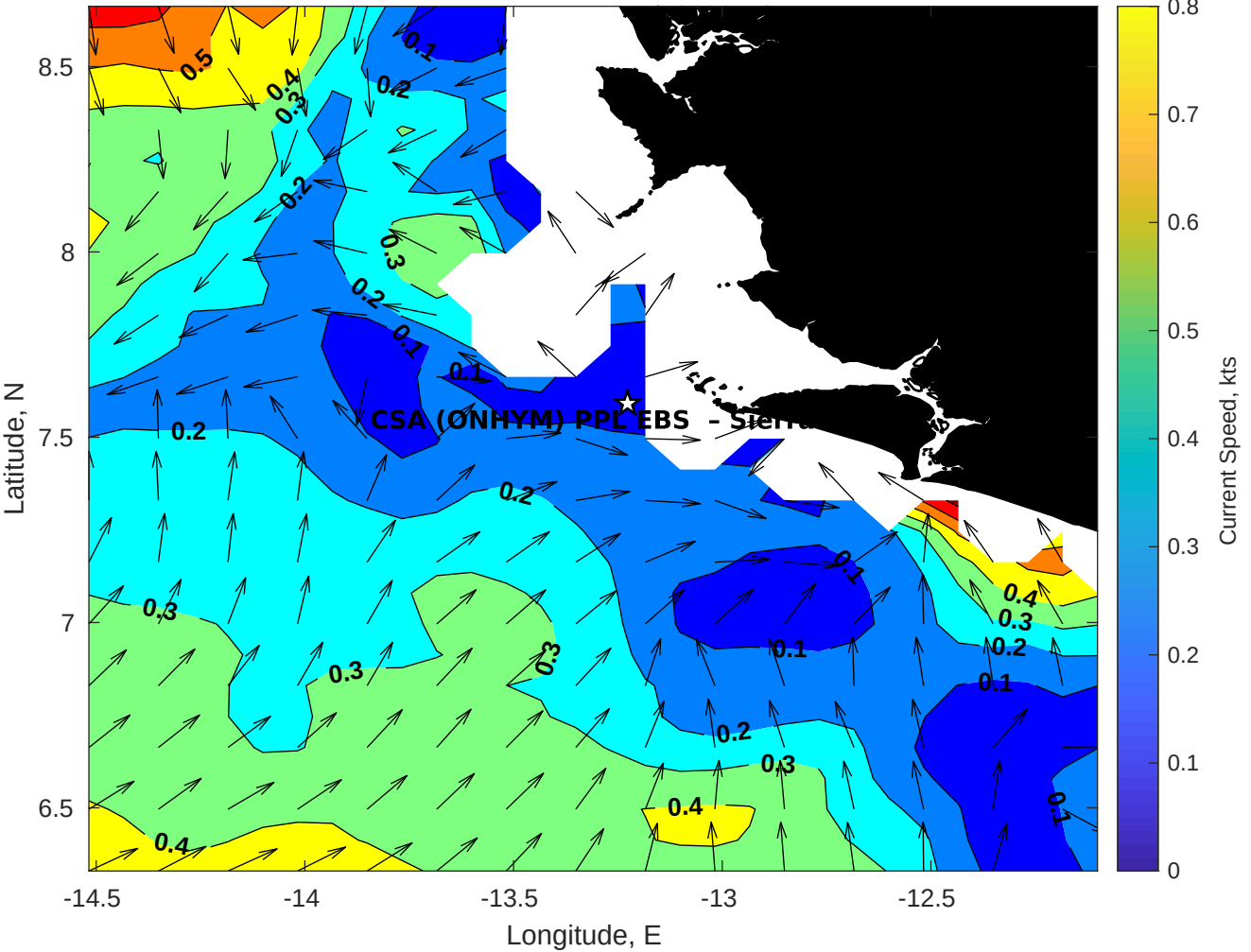
Surface Currents for CSA (ONHYM) PPL EBS - Sierra Leone at 16-Oct-2025 00:00:00
