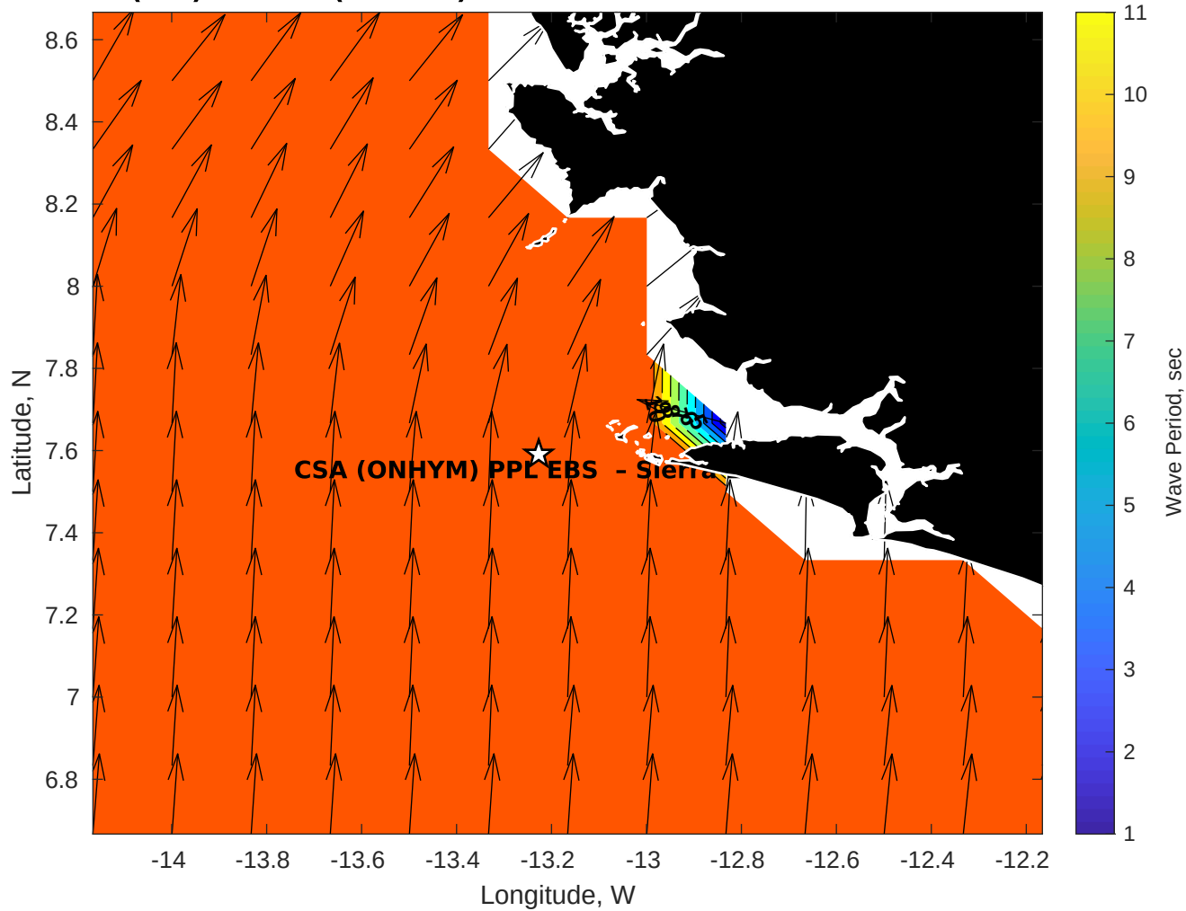
Wave Period (sec) for CSA (ONHYM) PPL EBS - Sierra Leone at 17-Oct-2025 09:00:00
