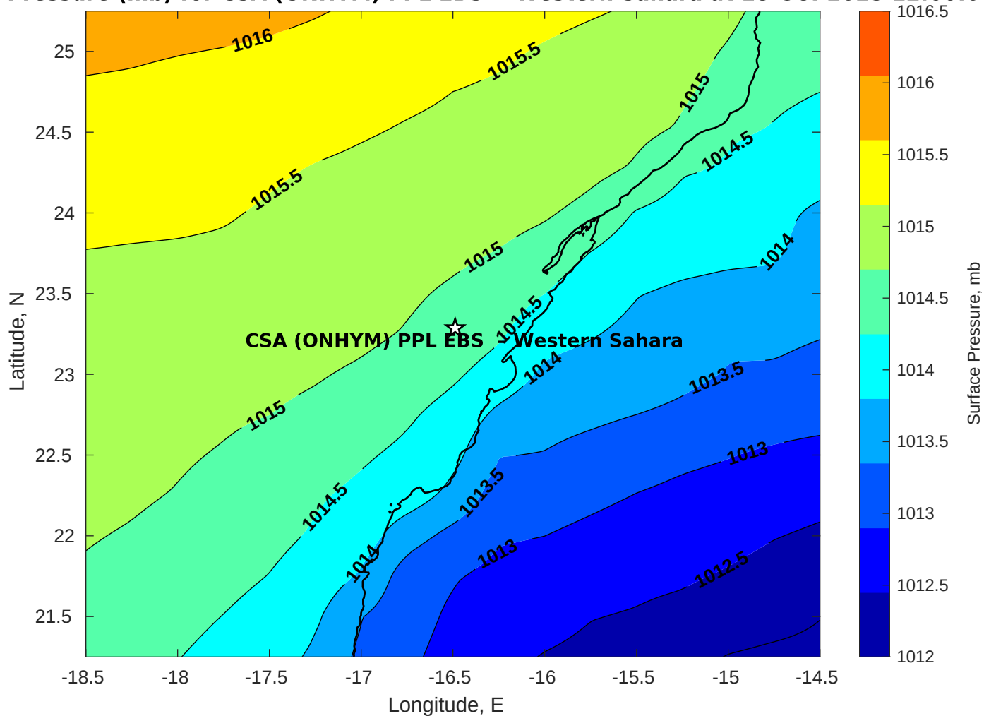
Surface Pressure (mb) for CSA (ONHYM) PPL EBS - Western Sahara at 18-Oct-2025 12:00:00
