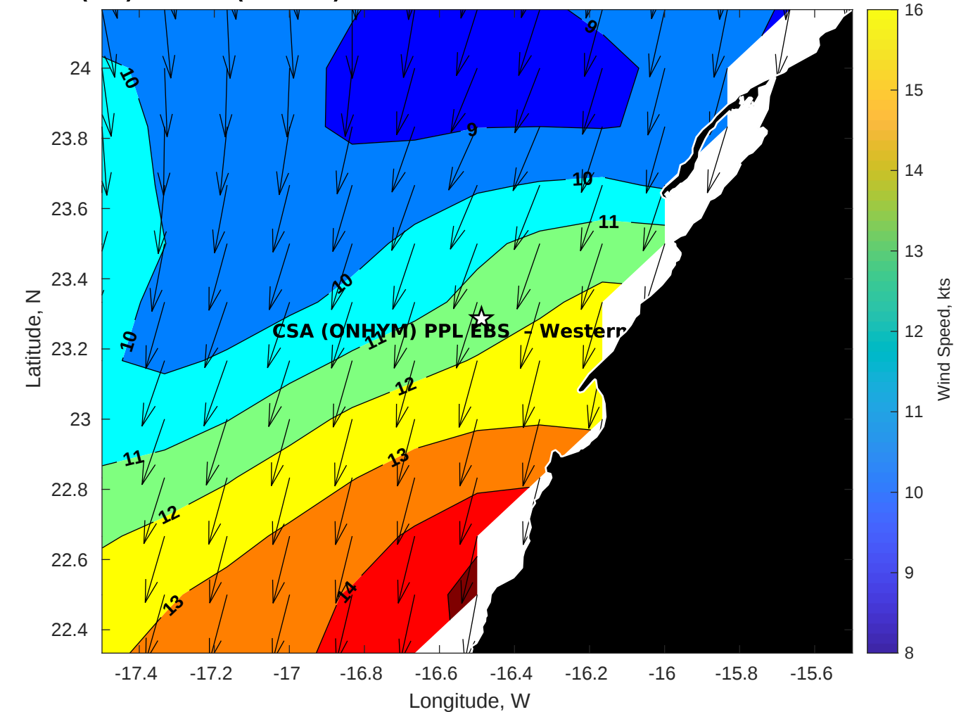
Winds (kts) for CSA (ONHYM) PPL EBS - Western Sahara at 16-Oct-2025 21:00:00
