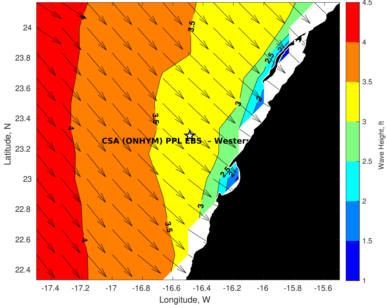
Wave Height (ft) for CSA (ONHYM) PPL EBS - Western Sahara at 16-Oct-2025 21:00:00
