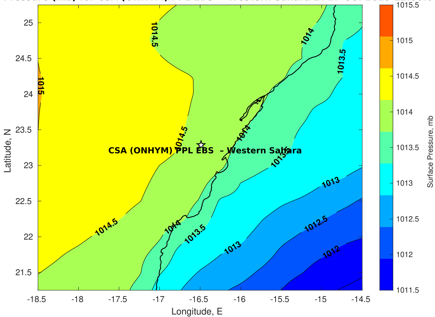
Surface Pressure (mb) for CSA (ONHYM) PPL EBS - Western Sahara at 17-Oct-2025 12:00:00
