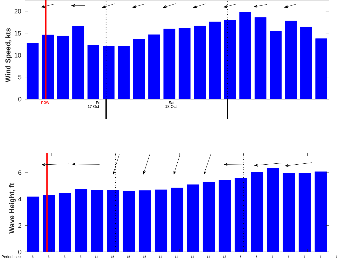
Wind & Wave Forecast for Gyre Passage: Dakar to Trinidad from 17-Oct-2025 07:00:00 to 19-Oct-2025 16:00:00
