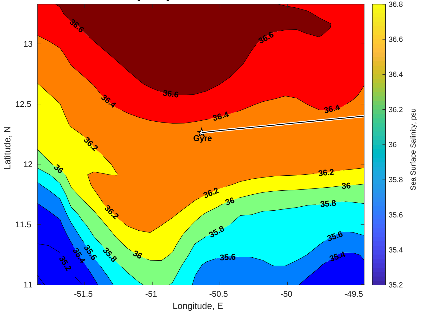
Surface Salinity for Gyre at 16-Oct-2025 00:00:00
