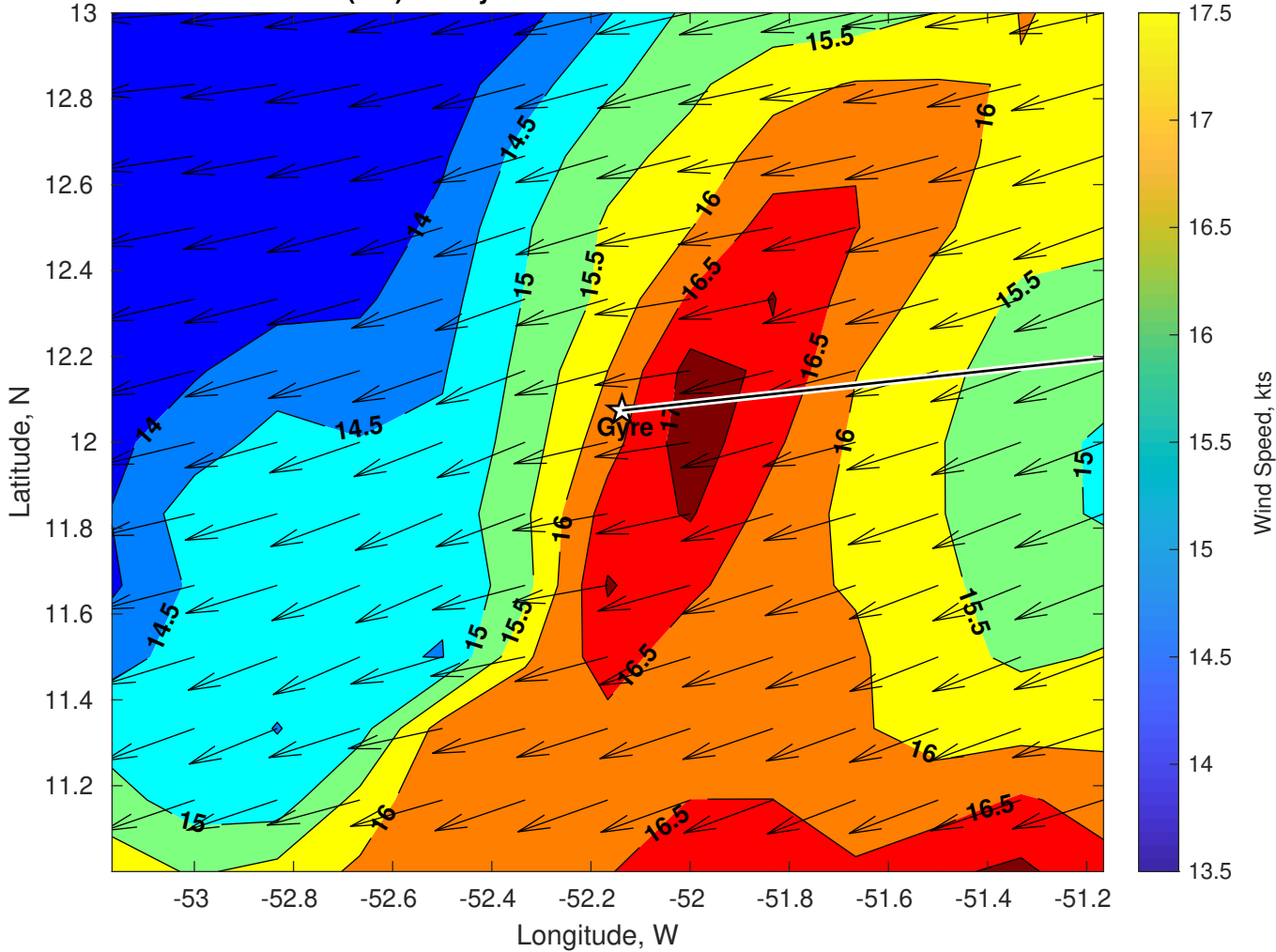
Winds (kts) for Gyre at 17-Oct-2025 09:00:00
