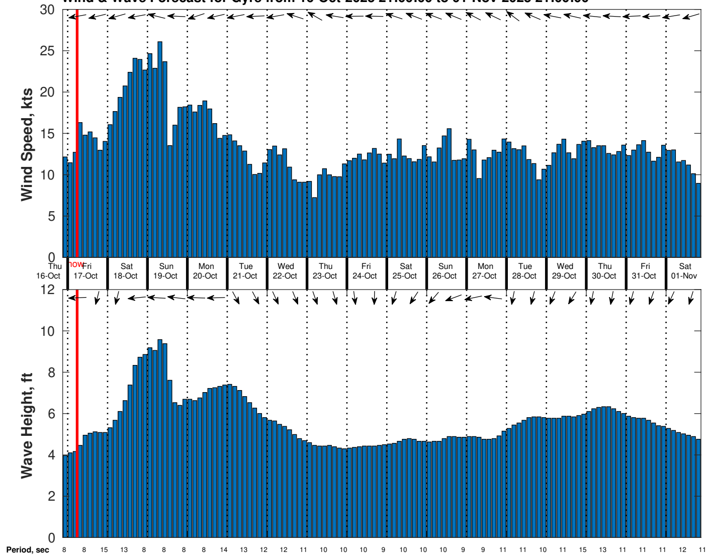
Wind & Wave Forecast for Gyre from 16-Oct-2025 21:00:00 to 01-Nov-2025 21:00:00
