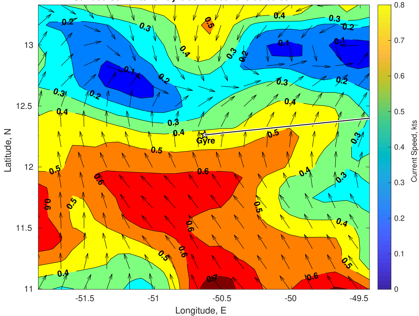
Surface Currents for Gyre at 16-Oct-2025 00:00:00
