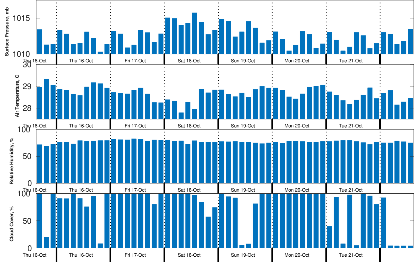
Met Forecast for Gyre from 16-Oct-2025 09:00:00 to 23-Oct-2025 09:00:00
