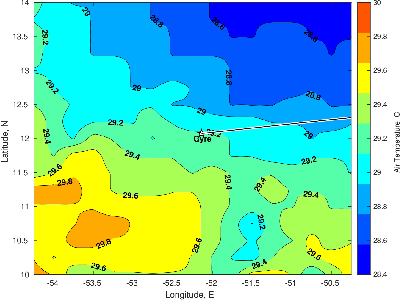
Air Temperature (C) for Gyre at 17-Oct-2025
