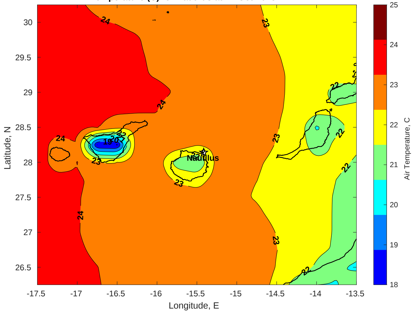
Air Temperature (C) for Nautilus at 17-Oct-2025
